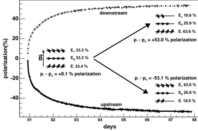
Figure 1. Typical deuteron polarization build up from 2004. Both upstream and downstream target cells are polarized simultaneously. About \pm 40\% polarization is reached in 24 hours after starting the microwave pumping of electron spins. The build up then slows down and the final polarization is reached in about 5 days from the beginning. The initial and final level populations for spin 1 deuteron are shown in the figure. The vector polarization P = p_- - p_+ is given by the population difference between the lowest and the highest energy levels. Since the gyromagnetic ratio of deuteron is positive the minimum energy E_- is achieved when the spin is aligned along the magnetic field. The tensor polarization can be estimated to be T = 1/2(1 - 3p_0) = 11\% at the maximum. The highest polarizations correspond to a spin temperature T_S of 0.87 mK or -0.87 mK for the negative polarization. From Eq. 2 the polarization of {}^6\text{Li} can be estimated to be \pm 51.3\% and the polarization of {}^7\text{Li} \pm 92.4\% .
