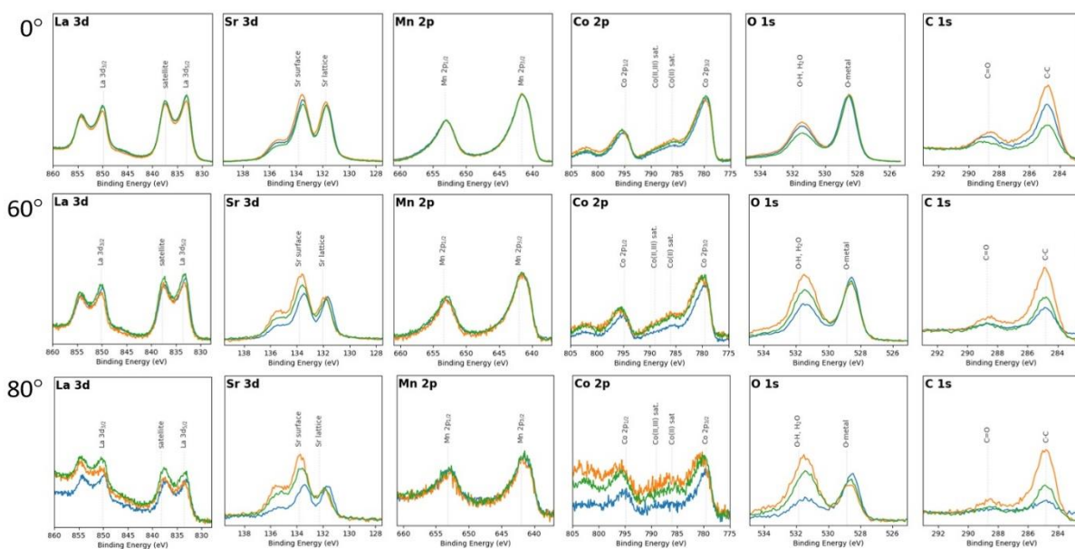
Figure S10. Angle-resolved XPS for LSMC/LAO (blue), LSMC/LSAT (green) and LSMC/STO (red) after Shirley correction and normalized to Mn 2p_{3/2} .
