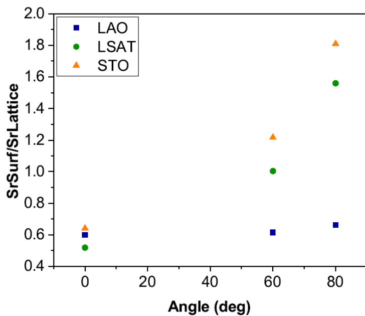
Figure 5. Ratio of Sr3d 5/2 signals for Sr-O lattice SrCO 3 surface peak areas at both angles normal (0°) and glancing to the surface (60° and 80°). The higher ratio at higher angles for LSMC/LSAT and LSMC/STO suggests greater strontium carbonate at the surface of films under tensile strain. The accuracy of XPS atomic concentrations is within 2% .
