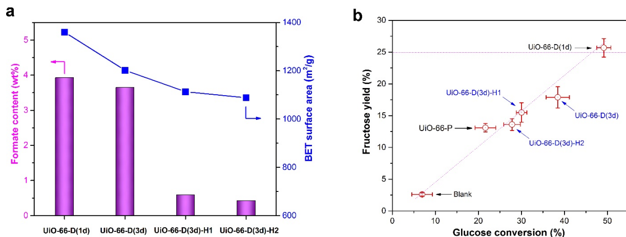
Figure 5 | Characterization and catalytic performances of various defective UiO-66 samples. a , Formate contents determined by high-performance liquid chromatography analysis of HF-digested solution (see the section of “Determination of the formate content in UiO-66 samples” in Supplementary Information for detailed method), and BET surface areas derived from N 2 sorption isotherms of four UiO-66 samples as labelled. b , Catalytic performances of various UiO-66 samples in the isomerization of glucose to fructose. “Blank” refers to the case without using a catalyst. The error bars represent standard uncertainties in the mean values calculated from five batches of repeated experiments.
