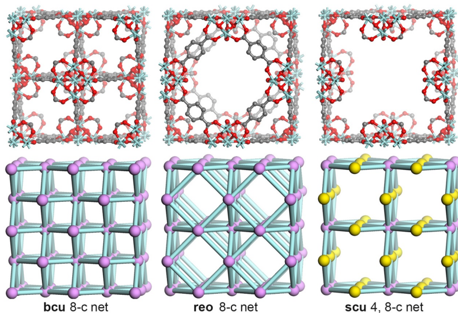
Figure 4 | Illustrations of various defective structures in UiO-66. (Top) crystallographic models and (Bottom) the corresponding topological representatives ( 2 \times 2 \times 2 ) of the 8-connected missing linker defects ( bcu net; transitivity [1112]), 8-connected missing cluster defects ( reo net; transitivity [1122]), and the 4,8-connected missing cluster defects ( scu net; transitivity [2133]). The transivities [pqrs] denote p types of vertices, q types of edges, r types of faces and s types of tiles. Pink and yellow balls indicate 8- and 4-connected nodes, respectively.
