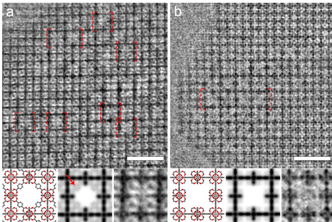
Figure 3 | HRTEM analysis of the “missing cluster” defects in UiO-66-D. CTF-corrected HRTEM images of the [001] direction, showing different types of missing cluster defects: (a) reo and (b) scu . In the bottom panel of each figure, from left to right, are the projected structural model, the simulated projected potential map, and the experimental image (processed by real space averaging to enhance the signal to noise ratio) for comparison. The unit cells used for averaging are labeled in the images with red dashed boxes. The scale bars represent 5 nm. The contrast associated with the BDC linkers surrounding the missing cluster is indicated by a red arrow in the simulated potential map in (a) .
