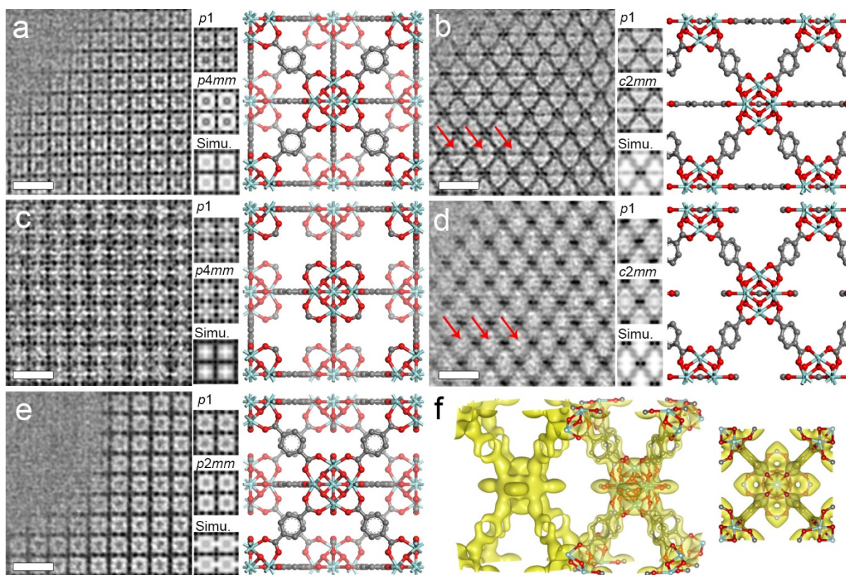
Figure 2 | HRTEM analysis of perfect and “missing linker” regions in UiO-66-D. a-e, CTF-corrected HRTEM images and structural models along the [001] (a) and [110] (b) zone axes of perfect UiO-66 ( Fm\bar{3}m ), and along the [001] (c), [100] (d) and [110] (e) zone axes of the missing linker defect ( I4/mmm ). In each panel, left, CTF-corrected image; middle, from the top-down are p1 -averaged image, symmetry-imposed image, and simulated projected potential; right, the projected structural model. The similarity between the p1 -averaged and symmetry-imposed images validates the symmetry determination. The similarity between the processed HRTEM image and the simulated projected potential in c, d and e validates the structural model of the missing linker defect. f, Reconstructed 3D electrostatic potential map viewed in different orientations with the structural model of the missing linker defect superimposed, showing an 8-connected network with the Zr_6O_8 clusters, BDC linkers and defect terminating ligands (formates) that are all well resolved. Hydrogen atoms in all structural models are omitted for clarity. The scale bars represent 2 nm.
