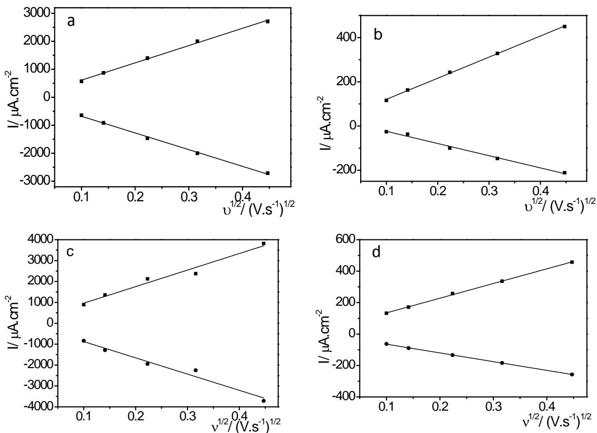
Figure 6: Randles-Sevcik plots obtained from voltammetric data for: a) GC in 10 mM \text{Fe}^{2+}/\text{Fe}^{3+} solution; b) GC in 1 mM dopamine solution; c) GC/SWCNT@SiO 2 in 10 mM \text{Fe}^{2+}/\text{Fe}^{3+} solution; d) GC/SWCNT@SiO 2 in 1 mM dopamine solution. Electrode geometric area: 0.07 cm 2 in all cases.
