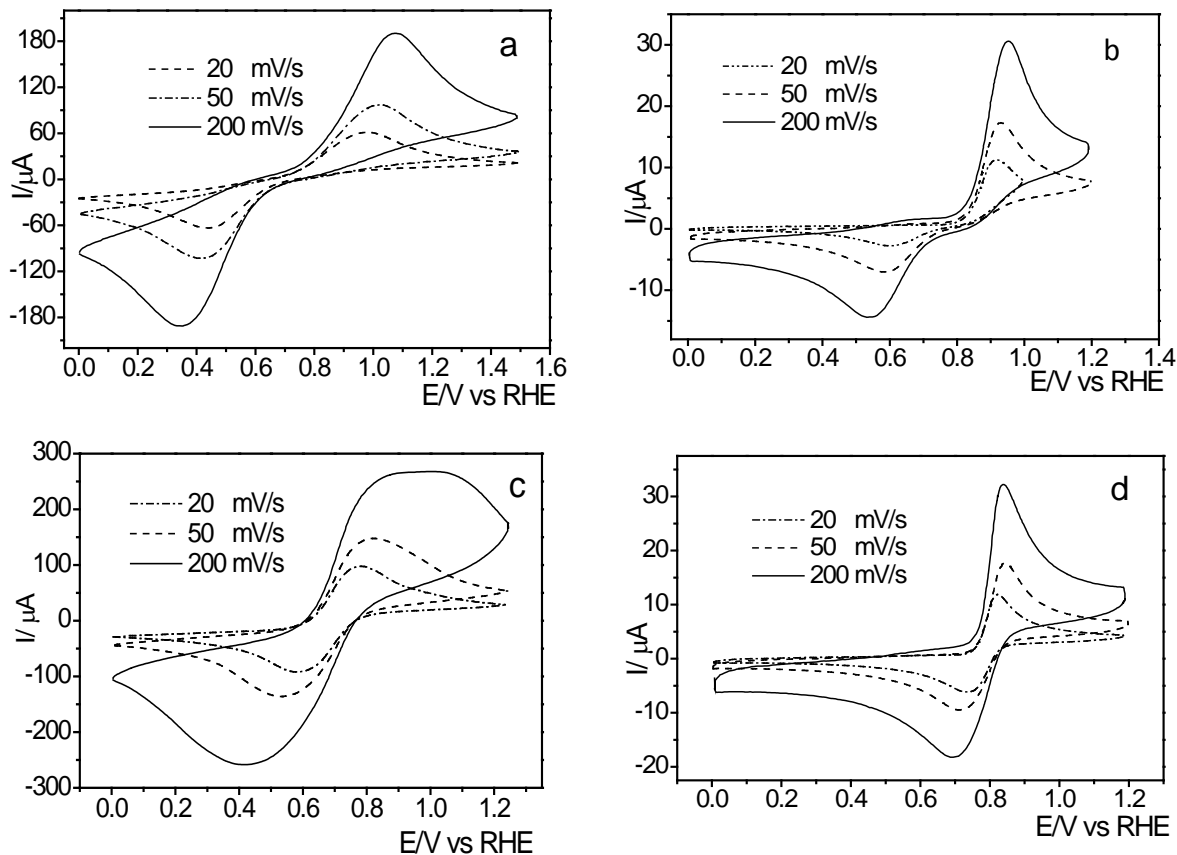
Figure 5: Steady state cyclic voltammograms recorded at different scan rates for: a) GC in 0.5 M H 2 SO 4 + 10 mM iron (II) sulfate/ 10 mM iron (III) sulfate solution; b) GC in 0.5 M H 2 SO 4 + 1 mM dopamine solution. c) GC/SWCNT@SiO 2 in 0.5 M H 2 SO 4 + 10 mM iron (II) sulfate/ 10 mM iron (III) sulfate solution; d) GC/SWCNT@SiO 2 in 0.5 M H 2 SO 4 + 1 mM dopamine solution. Electrode geometric area: 0.07 cm 2 in all cases.
