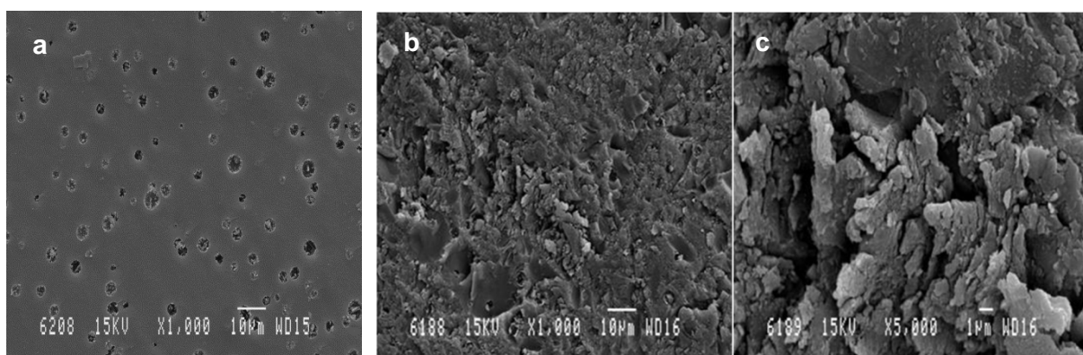
Figure 1: SEM micrographs acquired at different magnifications from: a) bare glassy carbon electrode, b) and c) glassy carbon substrate after the electroassisted deposition of the SWCNT@SiO 2 composite.
