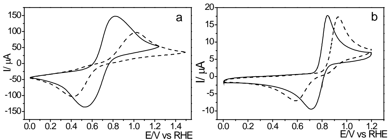
Figure 4: Stabilized cyclic voltammograms of glassy carbon electrodes (GC, dashed lines) or glassy carbon electrodes modified with single walled carbon nanotubes incorporated into silica layers (GC/SWCNT@SiO 2 , solid lines). Test solutions: (a) 0.5 M H 2 SO 4 + 10 mM iron (II) sulfate/ 10 mM iron (III) sulfate solution and (b) : 0.5 M H 2 SO 4 + 1mM dopamine solution; scan rate: 50 mV/s; electrode geometric area: 0.07 cm 2 .
