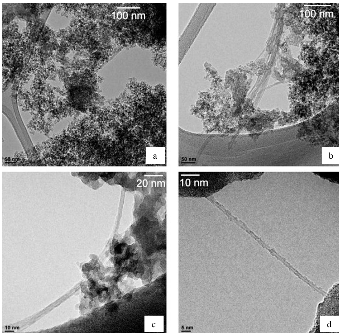
Figure 2. TEM micrographs of SWCNT@SiO 2 composites prepared by electroassisted deposition. (a) General view of the SWCNT@SiO 2 composite; (b) and (c) details of nanotubes bundles; (d) isolated SWNT found in-between SiO 2 aggregates.
