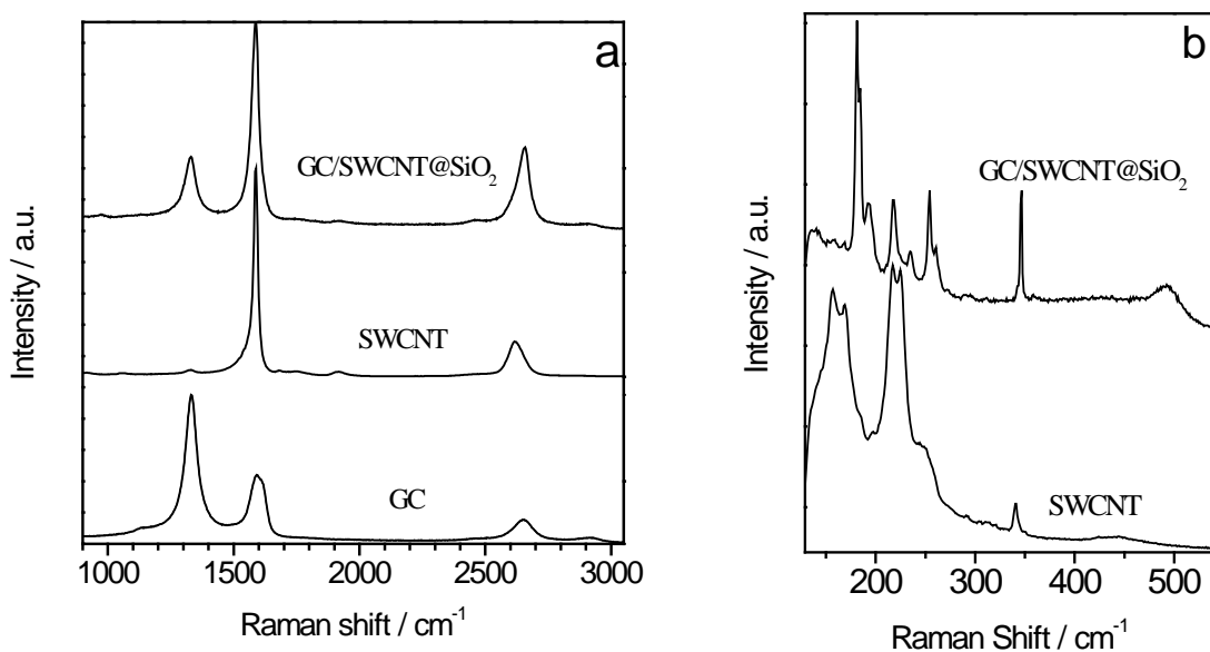
Figure 3: Raman spectra recorded (a) in the full frequency range and (b) RBM frequency region for: Bare glassy carbon electrode (labelled as GC), SWCNT powder from a DMF suspension (labelled as SWCNT) and SWCNT@SiO 2 prepared by electroassisted deposition deposited on a GC electrode (labelled as GC/SWCNT@SiO 2 ).
