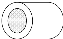
Figure 3. The grinding area must be slightly smaller than total face, in the case of a concrete core or specimen.
