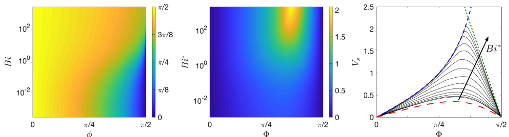
FIGURE 13. Calculations for a swimming cylindrical filament propelled by helical waves. (a) The pitch angle \Phi(\phi, Bi) , calculated from (4.10). (b) The swimming speed V_s(\Phi, Bi^*) . (c) The swimming speed for different Bingham numbers between Bi^* = 0.003 and Bi^* = 1995 , together with the Newtonian (red, long dashed) limit, the speed for perfect ‘corkscrewing’ (blue dashed), and the prediction for \Phi \rightarrow \pi/2 given in §4.3.3 (for \Omega \rightarrow 0 ; green, short dashed).
