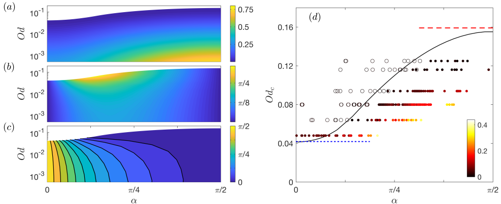
FIGURE 9. Numerical solutions for a cylinder whose axis is inclined at an angle of \frac{1}{2}\pi - \alpha to an applied force, with strength gauged by the Oldroyd number Od : (a) the fall speed V ; (b) the angle of motion \Psi = \phi - \alpha relative to the applied force; and (c) the angle of motion \pi/2 - \phi relative to its own axis. For Od > Od_c(\alpha) , the force on the cylinder is not sufficient to yield the fluid and there is no motion, leading to the white areas at the top of the plots. The critical value Od_c(\alpha) is shown in (d), together with the limits of transverse (short red dashed) and axial (long blue dashed) orientation, and a set of experimental data for headless machine screws sedimenting through a Carbopol gel (see Appendix D). Stationary rods are indicated by open circles and moving rods by filled circles, and the shading represents \sqrt{V} (in \sqrt{\text{cm/s}} ), according to the colour scheme indicated.
