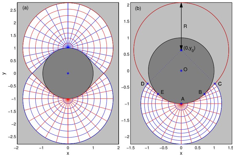
FIGURE 3. Slipline solutions for (a) \Omega = 0 and (b) \Omega = 1.6 . The two families of sliplines are shown with different colours ( \alpha -lines are red; \beta -lines are blue). Plugs are shaded light grey.
