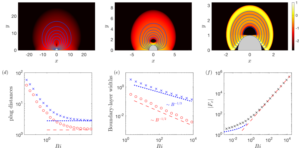
FIGURE 2. (a–c) Density plots of the logarithmic strain rate \log_{10}(\dot{\gamma}) in the (x, y) -plane (showing only y > 0 ), for a cylinder translating in the x direction ( \phi = 0 ), with (a) Bi = 0.0625 , (b) Bi = 1 , and (c) Bi = 1024 (note the different axis scales). The (blue) curves show streamlines, \psi = \text{constant} , in the frame of the ambient fluid. (d) The distance from the centre of the cylinder to the furthest yield surface along the x (red circles) and y (blue crosses) axes; the slipline predictions ( \sqrt{2} and 2 + \frac{1}{4}\pi ) are shown by dashed lines. (e) The widths of the boundary layer against the cylinder (red circles) and the outer free shear layer (blue crosses), both along x = 0 . (f) The force |F_x(Bi)| , together with the Newtonian (blue dots; (3.2a)) and plastic (red dashed; (3.11)) predictions.
