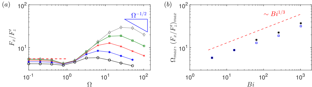
FIGURE 14. (a) Computations of the speed coefficient F_x(0, \Omega, Bi)/F'_z(\Omega, Bi) in (4.21) for varying \Omega and Bi = 4 (black circles), Bi = 16 (blue stars), Bi = 64 (red crosses), Bi = 256 (green squares) and Bi = 1024 (gray diamonds), together with the high-Bi limit for \Omega = 0 from the data in figure 8 (red dashed). (b) The (interpolated) maximum speed coefficient (F_x/F'_z)_{max} (blue squares) and corresponding Bingham number at which it is attained Bi_{max} (black stars).
