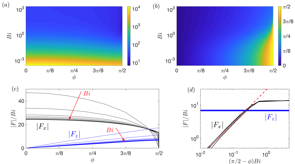
FIGURE 8. The drag force on a cylinder moving at an angle \phi to the x -axis. (a) The magnitude of the force, scaled by the Bingham number, |\mathbf{F}|/Bi . (b) The orientation of the force relative to the x -axis \alpha = \tan^{-1}(F_z/F_x) . Note that larger values of \alpha are confined to an increasingly narrow boundary layer for Bi \gg 1 . (c) The components of the drag F_x/Bi (black) and F_z/Bi (blue) for 1 \leq Bi \leq 2^{10} . (d) A magnification of the same data (showing 2^6 \leq Bi \leq 2^{10} ), for \phi \rightarrow \pi/2 . The red dashed line shows |F_x| = 9\pi(\pi/2 - \phi)Bi^2 (see Appendix C).
