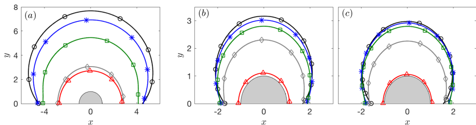
FIGURE 7. The outermost yield surface for (a) \text{Bi} = 1 , (b) \text{Bi} = 256 , and (c) \text{Bi} = 2048 . The surfaces correspond to inclination angles of \phi = 0 (black, circles), \phi = \pi/4 (blue, stars), \phi = 3\pi/8 (green, squares), \phi = 19\pi/40 (grey, diamonds) and \phi = \pi/2 (red, triangles).
