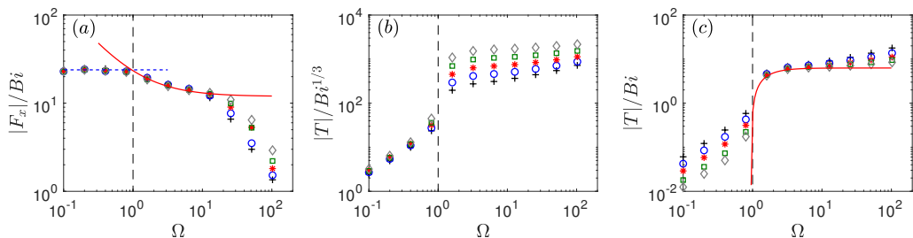
FIGURE 5. (a) Force and (b,c) torque for a cylinder translating with unit velocity in the x direction ( \phi = 0 ) and rotating with angular velocity \Omega . The data are scaled as indicated. The vertical dashed lines mark \Omega = 1 . Other lines show predictions for \text{Bi} \gg 1 : the horizontal dashed line in (a) shows the force for pure translation (3.11), and the red solid lines show the force and torque for solutions with a rigidly rotating upper plug (3.12). The different colours/symbols indicate data for \text{Bi} = 2^n with n = 8 (black cross), n = 9 (blue circle), n = 10 (red star), n = 11 (green square) and n = 12 (grey diamond).
