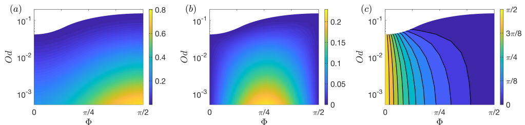
FIGURE 11. (a) The velocity V_s and (b) the angular rotation \omega for helix with pitch \Phi sedimenting along its axis. (c) The angle of motion \phi - \pi/2 of each filament of the helix to its own axial direction. Small angles indicate a nearly corkscrewing motion.
