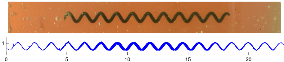
FIGURE 12. An image of a helix falling through Carbopol, and a plot showing successive snapshots of the centerline. The helix has mass M \approx 10.6 g, axial length 14 cm, radii \mathcal{R} \approx 1.2 mm and \mathcal{R}_H \approx 3.4 mm, pitch angle \Phi \approx 32^\circ , and falls vertically (to the right in the plots) with a speed of 0.83 cm/min.
