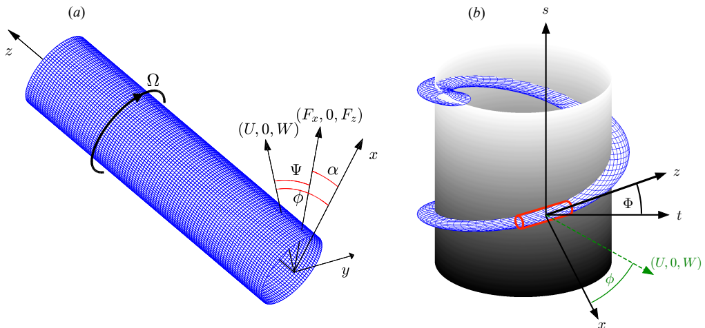
FIGURE 1. Sketch of the geometry: (a) the local cylindrical configuration. (b) a slender curved filament with circular cross section wrapped around another cylinder to form a helix.
