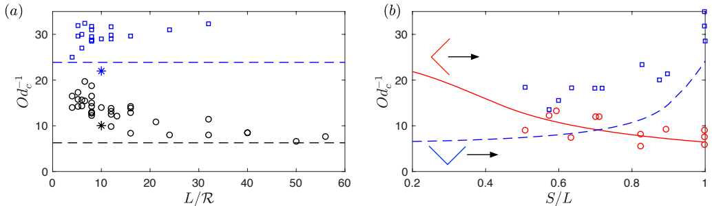
FIGURE 10. Comparison of experimental data from Madani et al. (2010) (points) with theory (lines) for the critical dimensionless force 1/\text{Od} at which cylinders of aspect ratio (length/radius) L/\mathcal{R} start to move. (a) Straight cylinders with axis aligned with the force (black circles) or side-on to the force (blue squares) together with our corresponding predictions for an infinite cylinder (dashed lines). The corresponding experimental results of Jossic & Magnin (2001) are also shown by stars. (b) Bent cylinders, in the orientations shown, where the force acts in the direction of the arrows, for different ratios of the shortest distance between ends S to the length L , together with the corresponding predictions (lines). The data are for cylinders with aspect ratios between L/\mathcal{R} = 20 and L/\mathcal{R} = 40 . All of the experimental data of Madani et al. (2010) has been divided by a factor of two.
