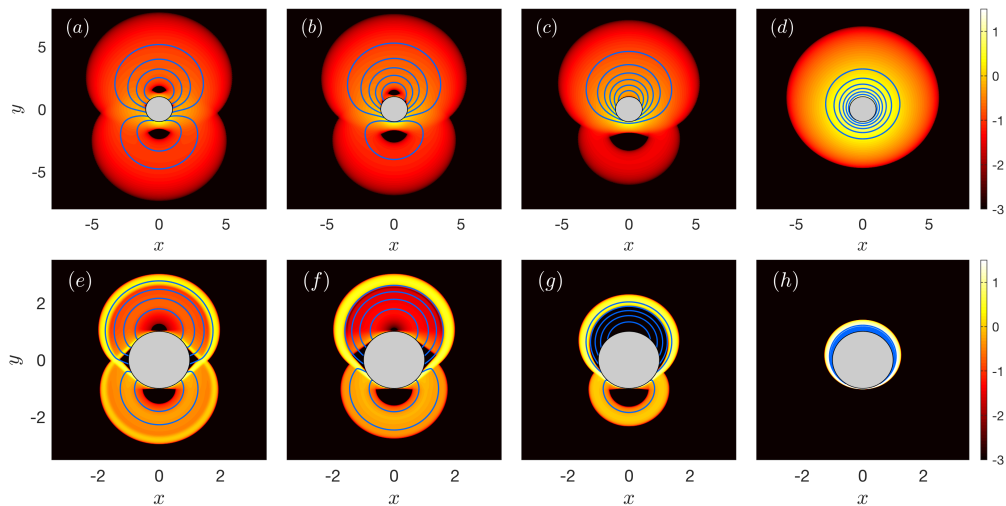
FIGURE 4. Density plots of \log_{10} \dot{\gamma} on the (x, y) -plane, overlain by streamlines, for a cylinder translating with unit velocity in the x direction ( \phi = 0 ) and rotating with angular velocity (a,e) \Omega = 0.4 , (b,f) \Omega = 0.8 , (c,g) \Omega = 1.6 and (d,h) \Omega = 12.8 . The upper row (a–d) is for \text{Bi} = 1 ; the lower row (e–h) is for \text{Bi} = 2048 .
