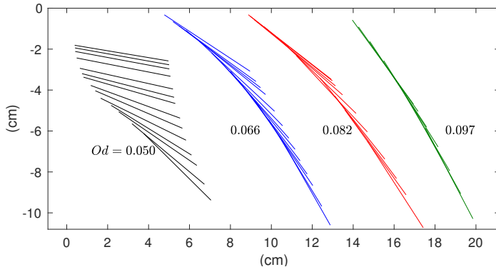
FIGURE 15. Snapshots (unequally spaced in time) of the centrelines of the four heaviest screws during sample falls. The spacing in time was roughly inversely proportional to the fall speed ( cf. figure 9d), and ranged from a few hundred seconds for the less tilted screws to a few seconds at higher inclinations.
