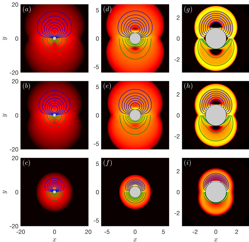
FIGURE 6. Density plots of logarithmic strain rate \log_{10}(\dot{\gamma}) for flow around non-rotating cylinders moving at an data areangle \phi , together with streamlines in the x - y plane ( i.e. \psi = \text{constant} ; blue, shown for y > 0 ) and contours of the axial velocity w (green, shown for y < 0 ). From left to right, the yield stresses are (a-c) B = 0.0625 , (d-f) B = 1 , and (g-i) B = 256 . From top to bottom, the angle of motion is (a,d,g) \phi = \pi/8 , (b,e,h) \phi = \pi/4 , and (c,f,i) \phi = 19\pi/40 .
