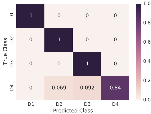
Figure 6: Confusion matrix for the identification of each phone at different locations through the city.
