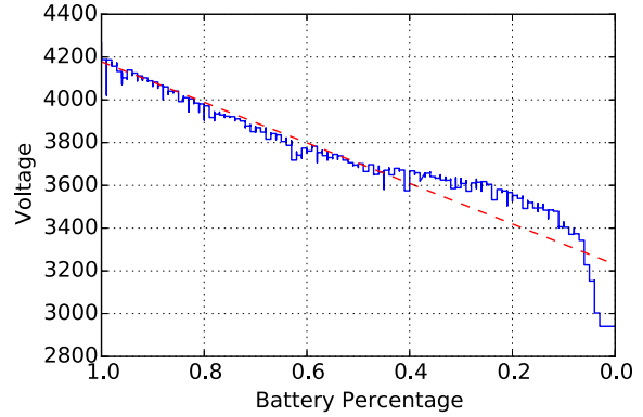
(b) Voltage as a function of battery consumption for a Motorola Nexus 6.
