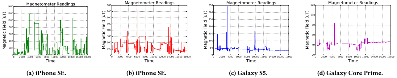
Figure 8: Magnetic field associated with four smartphones.
