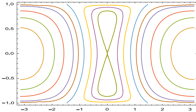
Fig. 2 Case \frac{1}{2} < \varepsilon < 1
