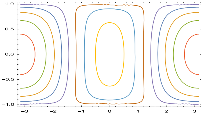
Fig. 1 Case 0 < \epsilon < \frac{1}{2}
