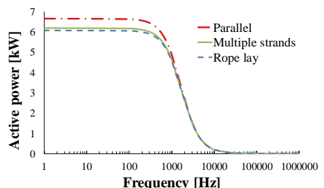
Fig.8. Frequency characteristic of active powers for three models when unit voltage is imposed
