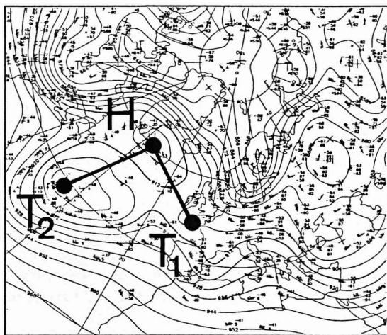
Geopotential 300 hPa am 27.03.96, 00 UTC
