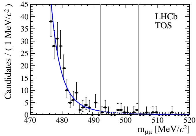
Fig. 2. – Background model fitted to data events which are triggered on the signal object (TOS), independently of the rest of the event. The vertical lines delimit the search region.
