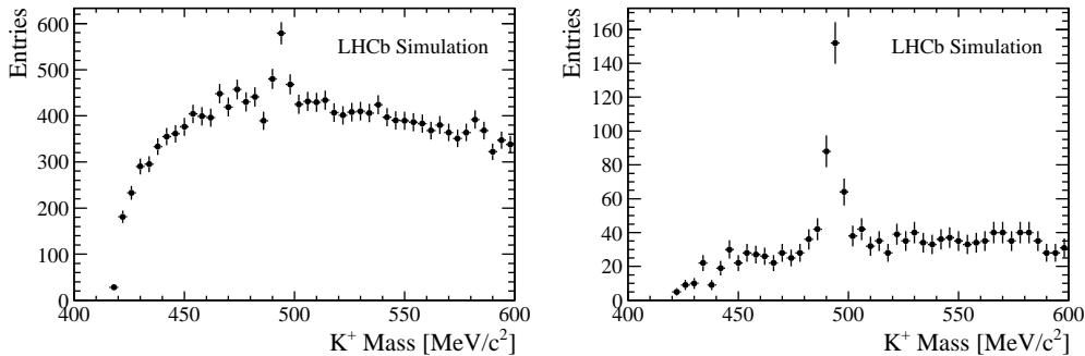
Fig. 4. – K^+ invariant mass distribution for simulated events. Left: no matching requirement applied. Right: after matching requirement.
