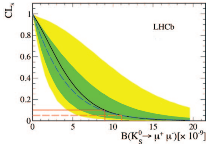
Fig. 3. – CLs curves. The solid line corresponds to the observed CLs. The dashed line corresponds to the median of the CLs for an ensemble of background-alone experiments. The dark band covers 65% ( 1\sigma ) of the CLs curves obtained in the background only pseudo-experiments, while the light band covers 95% ( 2\sigma ).
