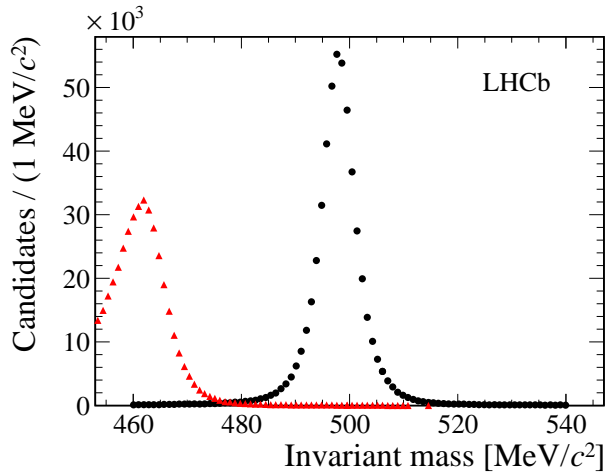
Fig. 1. – Mass spectrum for selected K_S^0 \rightarrow \pi^+\pi^- candidates. The points correspond to the mass reconstructed under the \pi^+\pi^- mass hypothesis for the daughters, while the triangles correspond to the mass reconstructed under the \mu^+\mu^- mass hypothesis.
