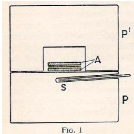
Fig. 4. – Apparatus for studying neutron absorption (Nuovo Cimento 12 (1935) p. 204).
