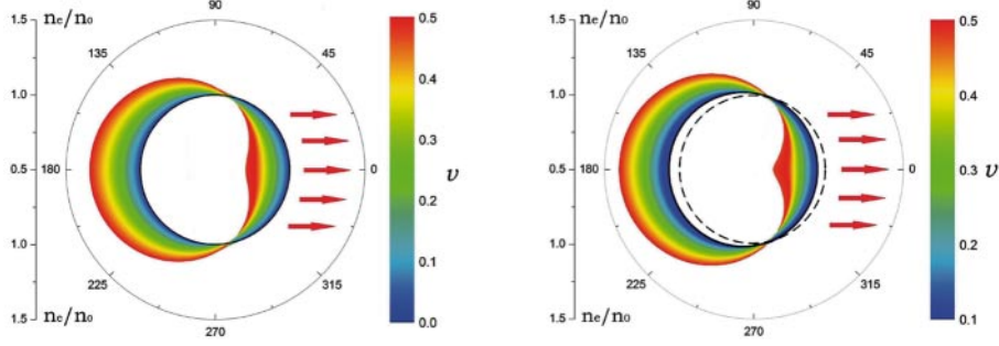
Fig. 1. – The figure illustrates distribution of the effective electron density in moving matter (normalized on the static value) as a function of matter speed v and the angle of propagation \phi . The red arrows define the direction of the neutrino flux. The left and right plots corresponds to v_0 = 0 and v_0 = 0, 1 accordingly.
