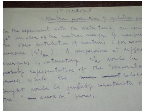
Fig. 3. – The first entry by Bruno in the 1950 secret logbook describing fundamental research with particles at the new accelerator.
