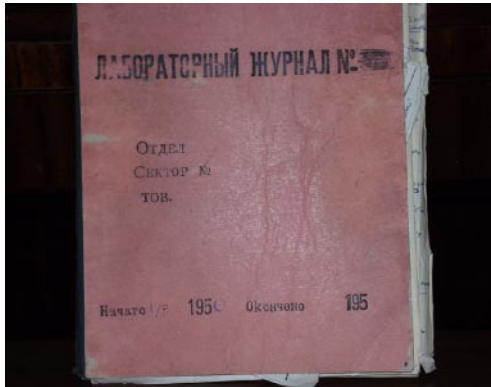
Fig. 2. – Secret logbook for recording the scientific lab work in Dubna in 1950, pages numbered! (Courtesy of JINR Archives).
