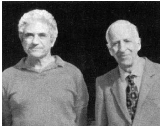
Fig. 9. – Bruno Pontecorvo (right) and Jack Steinberger in 1989.
