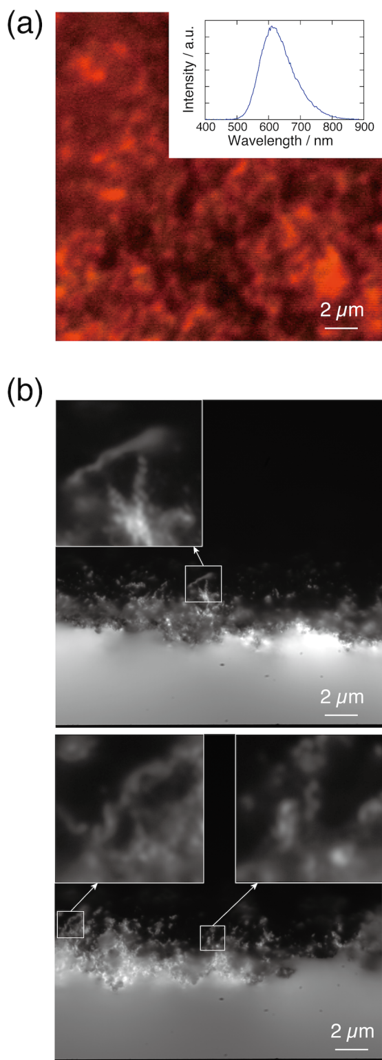
Fig. 3. (a) Photoluminescence from the top surface of the silicon substrate after PacEtch, together with the spectrum of the luminescence. Images in (b) show the photoluminescence from the cross-section observed using a microscope. In the magnified images, luminescence shows helical shapes, suggesting that microporous silicon remains on the wall surface of the helical pores.
