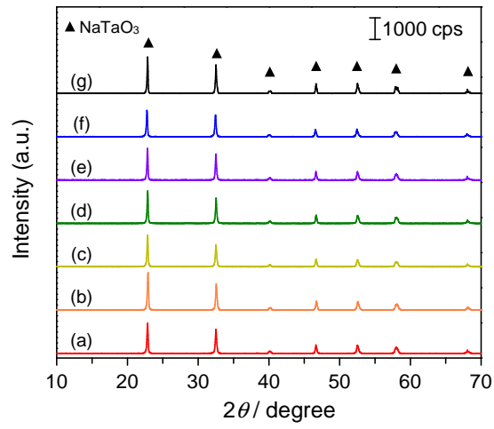
Fig. 2. XRD patterns of the \text{Pt}(0.03)/\text{NaTaO}_3:\text{La}(x,1273,2) samples prepared by the flux method at various solute concentrations of (a) 5, (b) 30, (c) 50, (d) 70, (e) 90, and (f) 100 mol%, and (g) the \text{Pt}(0.03)/\text{NaTaO}_3(70,1273,0) sample without La doping. The \text{NaTaO}_3:\text{La}(100,1273,2) sample was prepared without the flux.
