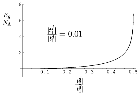
FIG. 2. Ground-state energy per lattice site, Eq. (25), in units of U as a function of y=|t_2^d/t_1^d| for the localized solution in a simple cubic crystal for |t_1^f/t_1^d|=0.01 . As seen from the plot, E_g/N_\Lambda is finite at y_c=1/2 but has infinite slope.
