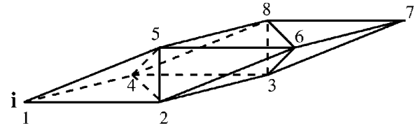
FIG. 4. Tilted unit cell located at site \mathbf{i} discussed in Sec. IV B. Number represent the intracell numbering of lattice sites. Only those bonds are presented along which hopping of d electrons occurs.
