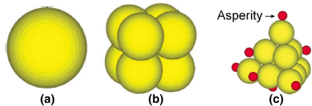
Fig. 9 Model of ballast particle as a sphere, b cubical cluster of 8 spheres, c tetrahedral clump of 10 un-breakable spheres with 8 breakable asperities [178]
