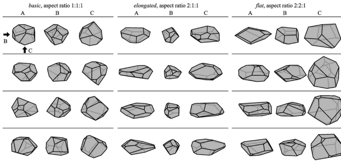
Fig. 12 Modelled ballast shapes as polyhedral particles generated randomly via Voronoi tessellation for three aspects ratios shown in front, side and bottom views A, B and C respectively [163]
