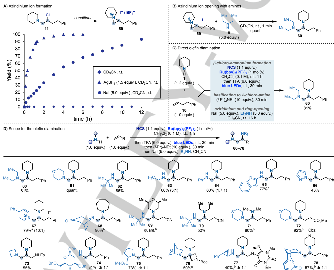
Scheme 4. (A) Reaction profiles for the formation of aziridinium 59 from 11 . (B) Aziridinium ring opening with Et 2 NH 8 is immediate. (C) Development of a procedure for direct olefin diamination. (D) Substrate scope for the direct olefin diamination using a range of different amine and olefin building blocks. * Denotes the minor constitutional isomer.
