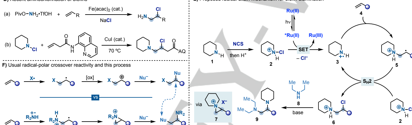
Scheme 1. (A) Vicinal diamines are high-value materials impacting many chemical sciences. (B) Current olefin diamination strategies do not enable the direct use of alkylamines. (C) The construction of unsymmetrical diamines requires multi-step syntheses while the strategy reported here assembles them in a single step. (D) Recent developments for olefin aminochlorination. (E) The proposed mechanism for olefin diamination involves the generation of an aminium radical to achieve an aminochlorination reaction which is followed by aziridinium formation and regioselective ring-opening. (F) This radical-polar crossover strategy offers a different disconnection to classical approaches.
