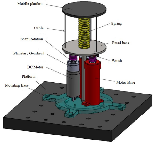
Figure 1: Prototype functional scheme.
