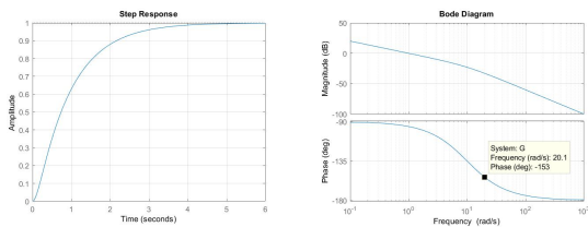
Figure 5: Step response of the motor (left). Bode diagram of the motor (right).
