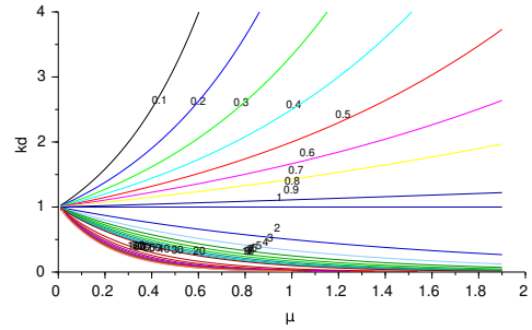
Figure 9: Parameter tuning plot, showing iso_\omega curves as a function of \mu and k_d .
