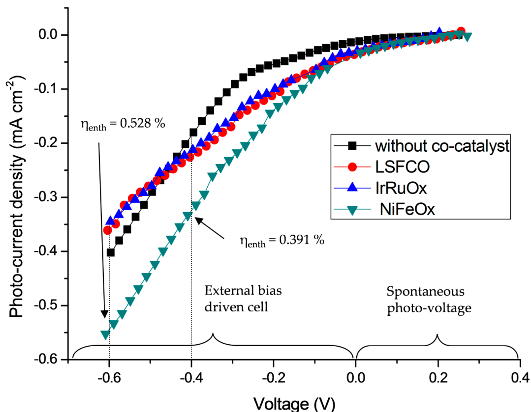
Figure 3. Polarization of the photocurrent for 4 PECs, without any co-catalyst addition and with the IrRuOx, LSFÇO and NiFeOx co-catalyst-based photoanodes.
