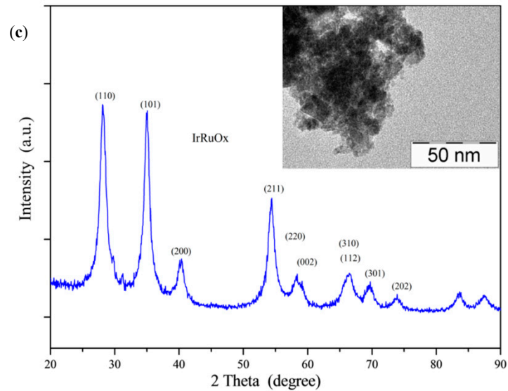
Figure 1. XRD tests and TEM images in the inset for (a) NiFeOx, (b) La 0.6 Sr 0.4 Fe 0.8 Co 0.2 (LSFCO) and (c) IrRuOx.
