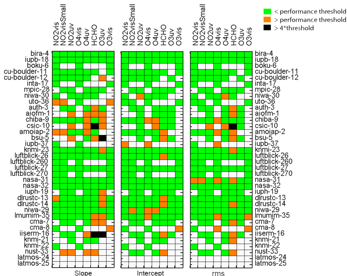
Figure 20. Overview of performance results for the slope, intercept and rms from the regression analysis displayed for all participating instruments and MAX-DOAS data products. Colour coding denotes whether each of the parameters is within the set criteria (green), whether the performance threshold is exceeded (orange), or whether it is exceeded by more than a factor of 4 (black).
