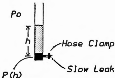
Figure 3. Rubber hose and hose clamp apparatus used in the second experiment. P_0 is the external air pressure and P(h) is the water pressure at the depth h .
