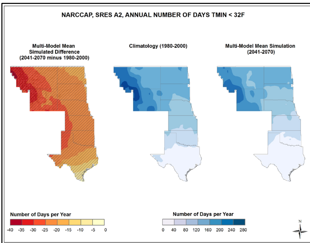
Figure 19. Simulated difference in the mean annual number of days with a minimum temperature less than 32°F ( T_{min} < 32^{\circ}\text{F} ) for the Great Plains region, for the 2041-2070 time period with respect to the reference period of 1980-2000 (left). Color with hatching (category 3) indicates that more than 50% of the models show a statistically significant change in the number of days, and more than 67% agree on the sign of the change (see text). Mean annual number of days with T_{min} < 32^{\circ}\text{F} for the 1980-2000 reference period (center). Simulated mean annual number of days with T_{min} < 32^{\circ}\text{F} for the 2041-2070 future time period (right). These are multi-model means from 8 NARCCAP regional climate simulations for the high (A2) emissions scenario. Changes are downward everywhere. Decreases are largest in the northwest of the region and smallest in the far south.
