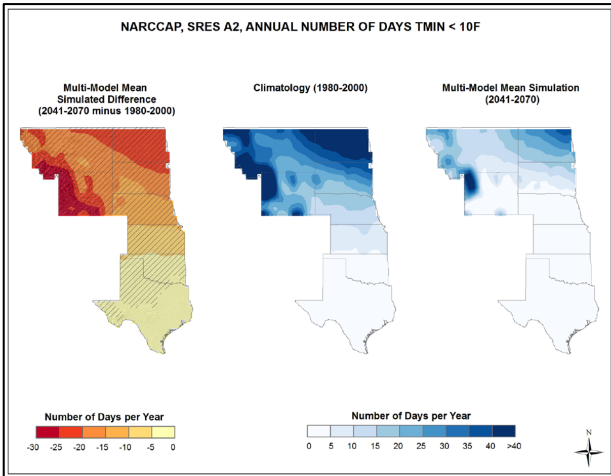
Figure 18. Simulated difference in the mean annual number of days with a minimum temperature less than 10°F ( T_{min} < 10^{\circ}F ) for the Great Plains region, for the 2041-2070 time period with respect to the reference period of 1980-2000 (left). Color only (category 1) indicates that less than 50% of the models show a statistically significant change in the number of days. Color with hatching (category 3) indicates that more than 50% of the models show a statistically significant change in the number of days, and more than 67% agree on the sign of the change (see text). Mean annual number of days with T_{min} < 10^{\circ}F for the 1980-2000 reference period (center). Simulated mean annual number of days with T_{min} < 10^{\circ}F for the 2041-2070 future time period (right). These are multi-model means from 8 NARCCAP regional climate simulations for the high (A2) emissions scenario. Decreases are largest in the north and in high elevation areas, and become smaller southward, in a pattern similar to the present-day climatology.
