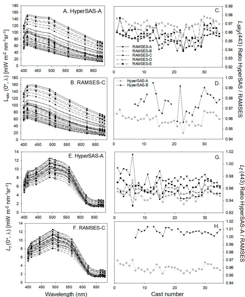
Figure 11. L_{sky} spectra of all casts for (A) HyperSAS-A, (B) RAMSES-C, and for each cast over time as the ratio of (C) L_{sky}(443) for HyperSAS-A / each RAMSES system and (D) HyperSAS-A and -B/mean of RAMSES systems (RAMSES-A, -B, -C, -D, -E). L_t spectra of all casts for (E) HyperSAS-A, (F) RAMSES-C, and for each cast over time as the ratio of (G) L_t(443) for HyperSAS-A/each RAMSES system and (H) HyperSAS-A and -B/mean of RAMSES systems (RAMSES-A, -B, -C, -D, -E).
