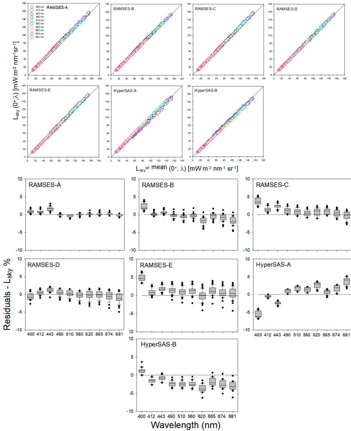
Figure 7. Top Panel: Scatter plots of L_{sky} at 90° and 135° relative azimuth from the different above-water systems versus weighted mean L_{sky} ( L_{sky}^{wt \text{ mean}} ) from above-water systems (RAMSES-A, -B, -C, HyperSAS-A, -B). The different coloured points correspond to the different OLCI bands given in the RAMSES-A subplot. Bottom Panel: Residuals of L_{sky} expressed as a percent for the different above-water systems. The residuals at each wavelength are calculated from each system [(L_{sky} - L_{sky}^{wt \text{ mean}})/L_{sky}^{wt \text{ mean}}]*100 .
