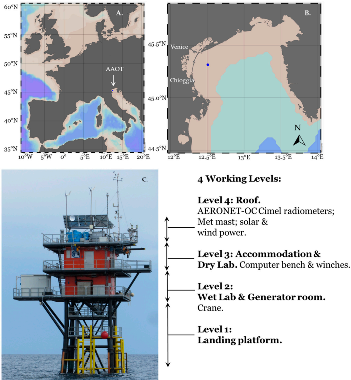
Figure 1. (A) Map showing the location of the Acqua Alta Oceanographic Tower (AAOT) in Europe and (B) in the Northern Adriatic Sea; (C) schematic of the AAOT. For the intercomparison, the
