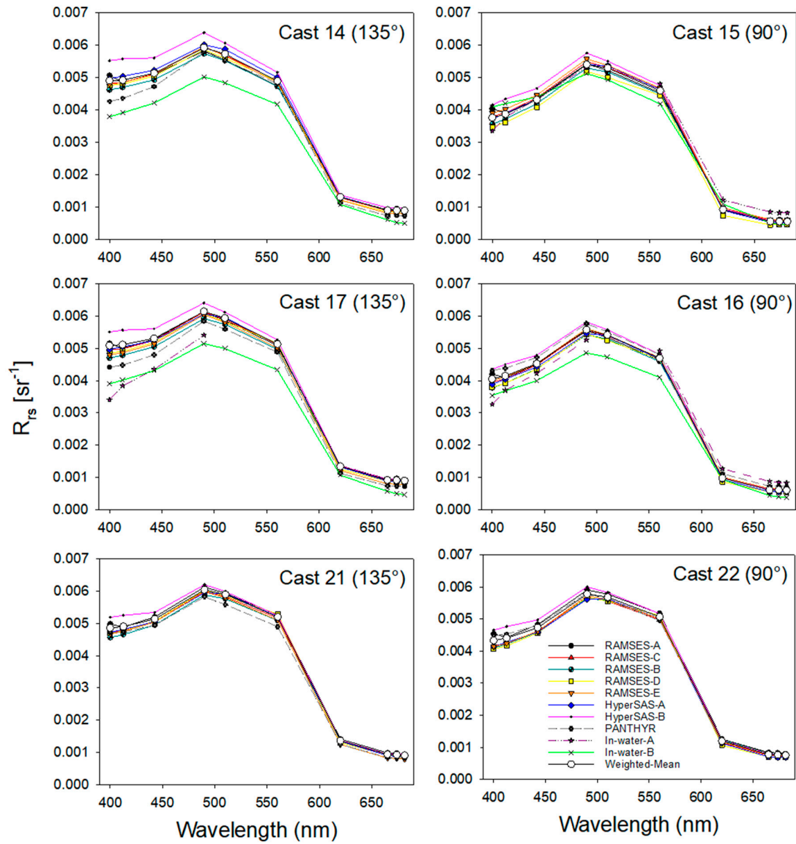
Figure A6. Variation in R_{rs} spectra of all instrument systems at OLCI bands for Casts with adjacent viewing angles at 135^\circ and 90^\circ on 14 July 2018.
