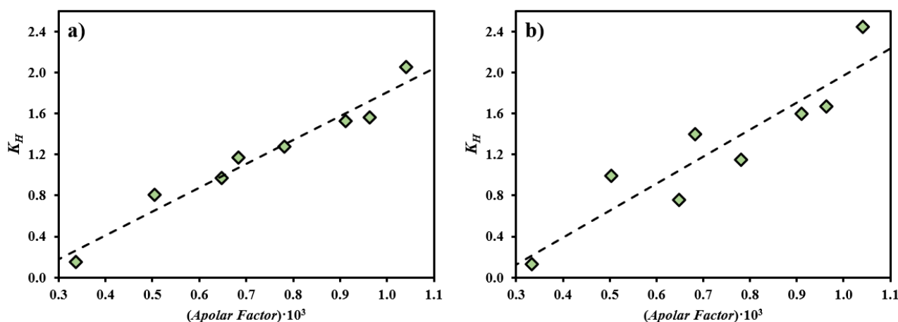
Figure 2. Setschenow constants 16 for a) gallic acid or b) syringic acid in glycerol ether-based hydrotropic solutions as a function of the apolar factor of the hydrotrope. The dashed line is the straight line fitted to the data using the least squares method.
