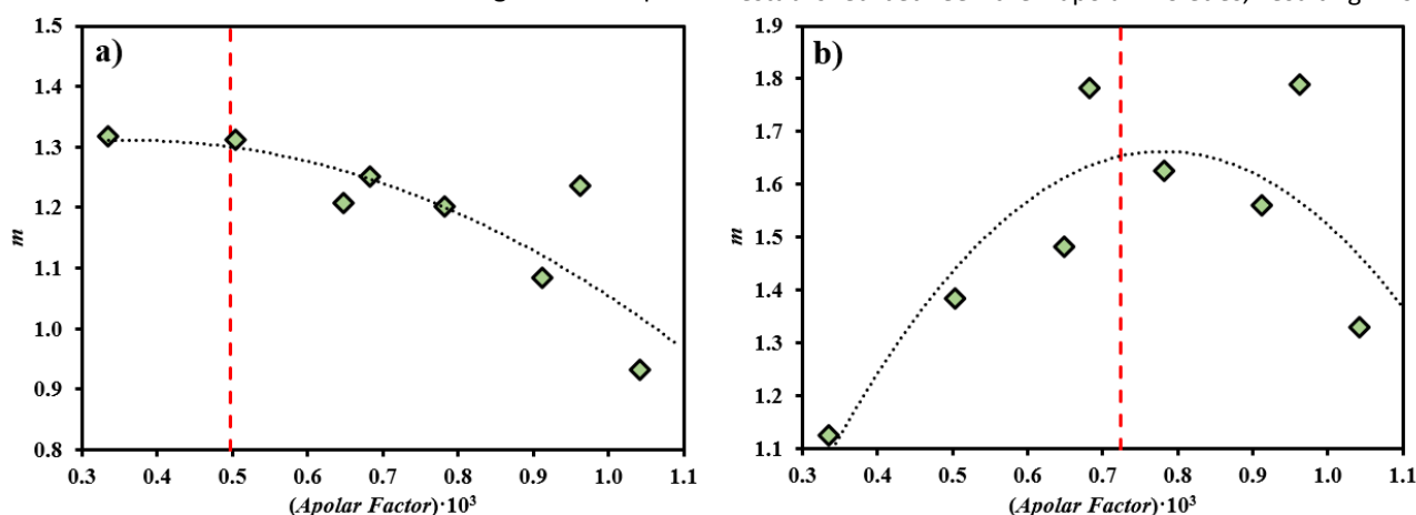
Figure 3. Dependency of the number of hydrotrope molecules in the vicinity of the solute ( m ) on the apolar factor of the hydrotrope, estimated using the Shimizu and Matubayasi 19 model for a) gallic acid and b) syringic acid in aqueous solutions of glycerol ethers 16 . The black dashed line is a visual guide whilst the red dashed line represents the apolar factor of the solute.
