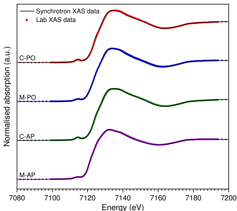
Figure 2. Comparison of normalised transmission mode Fe K-edge XANES spectra from 40\text{Fe}_2\text{O}_3\text{-}60\text{P}_2\text{O}_5 glasses prepared by microwave (M) or conventional (C) heating of \text{Fe}_3\text{O}_4 with \text{P}_2\text{O}_5 (PO) or \text{NH}_4\text{H}_2\text{PO}_4 (AP), acquired using laboratory XAS spectrometer (points) and KMC-2 synchrotron beamline (solid line).
