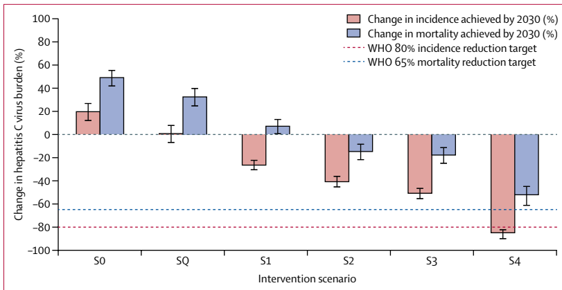
Figure 2: Relative change in incidence and mortality achieved by 2030 versus 2015, by intervention scenario. Data are the median of 1151 final model runs. Error bars are 95% uncertainty intervals. Scenario S0: no screening or treatment from 2018 onwards. Scenario SQ: maintaining status quo treatment of 150 000–160 000 annual treatments from 2018. Scenario S1: one-time random screening of 90% of the general population of Pakistan by 2030, with 80% referral to care. Scenario S2: scenario S1 plus prioritised screening of people aged \geq 30 years and PWID. Scenario S3: scenario S2 plus rescreening of cured and previously antibody-negative or RNA-negative individuals from 2020 (every 10 years for non-PWID and annually for PWID). Scenario S4: scenario S3 with incremental improvements to achieve elimination. PWID=people who inject drugs.
