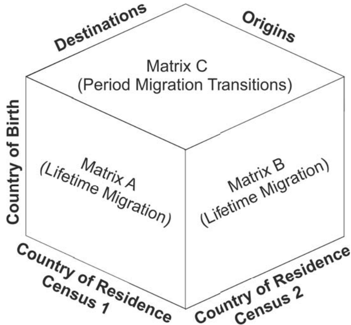
Fig. 3: A framework for estimating period migration from lifetime migration
