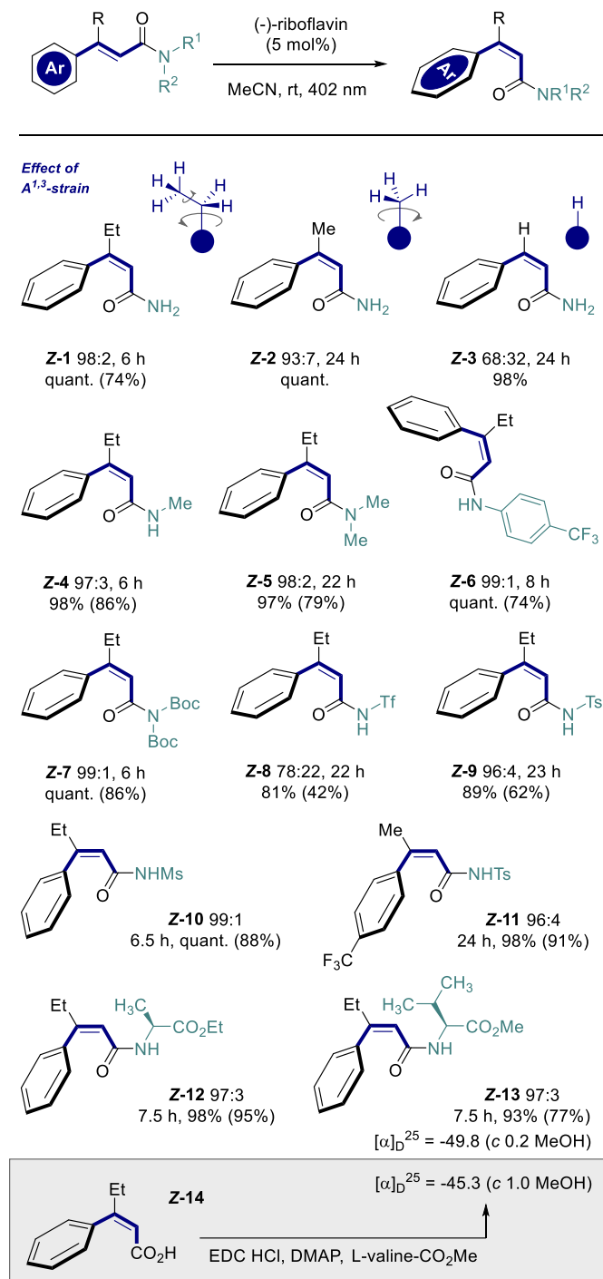
Fig. 2. Exploring the scope of the geometric isomerisation of cinnamamides using (–)-riboflavin. Reactions were performed on 0.1 mmol scale ( E / Z substrate >20:1) with 5 mol% (–)-riboflavin in 1.5 mL MeCN at ambient temperature ( \lambda = 402 nm); combined yields are given (isolated yields of the Z -isomer in parentheses). Bottom: Ensuring that optical purity is not compromised under the photoisomerization conditions.
