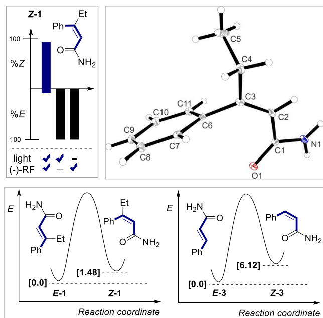
Figure 4. Top: Stern-Volmer photo-quenching study of E -1 and Z -1; Center left: Control experiments. Center right: X-ray crystal structure of Z -1 showing 1,3-allylic strain and intermolecular hydrogen bonding in the dimer (CCDC 1951608). Bottom: Lowest energy conformations of E -1 / Z -1 and E -3 / Z -3 at the [DG298/(kcal/mol)] (PWPB95-D3+CPCM(MeCN)//TPSS-D3) level of theory (please see the Supporting Information).
