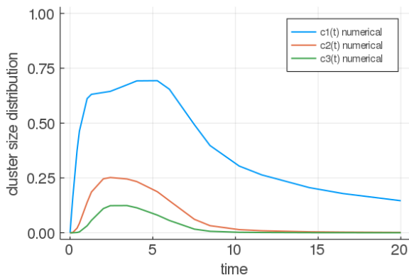
(a) \mu = 0, \nu = 1
