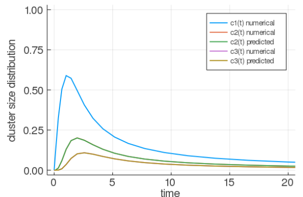
(c) \mu = \nu = 1.0
