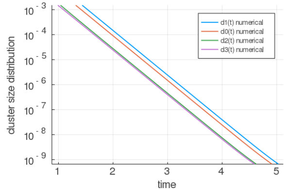
(b) \mu = 2, \nu = 0
