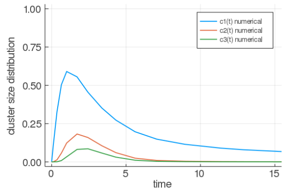
(b) \mu = 0, \nu = 1
