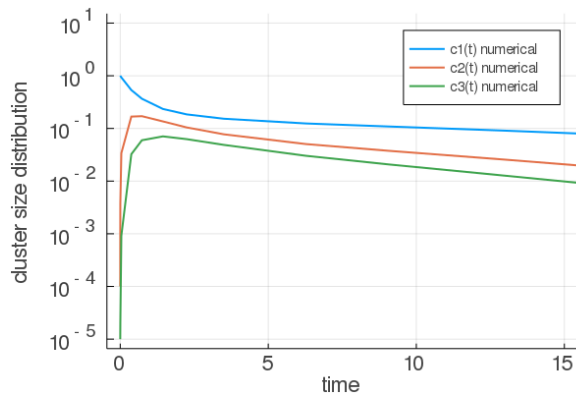
(a) \mu = 0, \nu = 1
