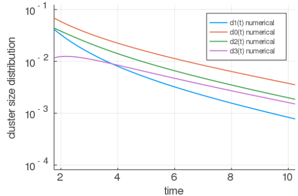
(a) \mu = 0, \nu = 0
