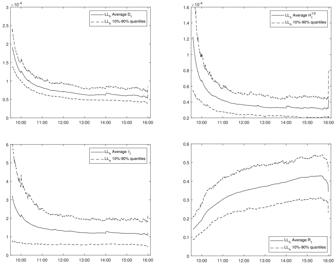
Figure 6: Average intraday patterns of the estimated LL_h time-varying parameters D_t, H_t^{1/2}, \delta_t and R_t . For each t = 1, \dots, 23400 , we report 10% and 90% quantiles of the distribution (over days) of averages of D_t, H_t^{1/2}, \delta_t and R_t (over assets or couples of assets).
