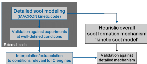
Figure 3: Flow chart of the kinetic soot model
