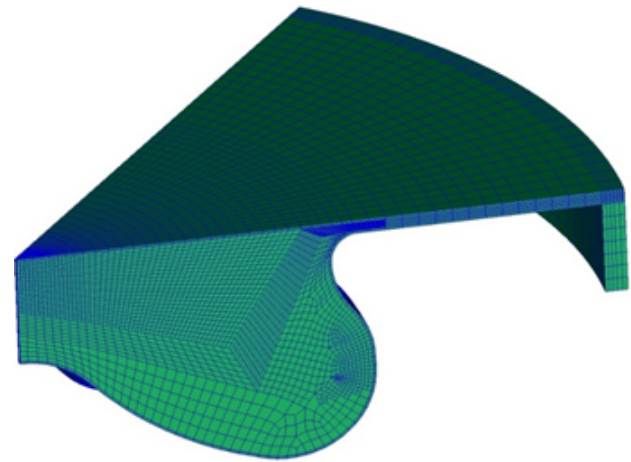
Figure 11: Computational (sector) mesh
