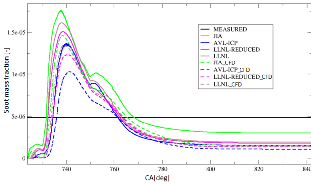
Figure 12: Comparison of soot mass fraction for the different mechanism used
