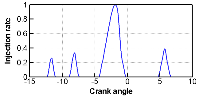
Figure 10: Injection timing
