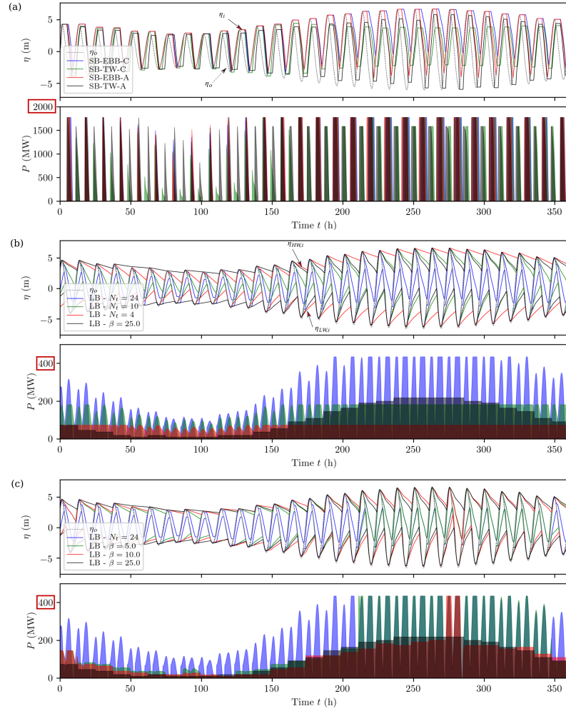
Figure 7: Elevations and power output of single- and linked-basin cases over a spring-neap cycle as predicted by 0D modelling. (a) Single-basin cases; (b) Comparison of linked-basin cases using a fixed number of turbines - including the adaptive operation linked-basin case with \beta = 25.0 (LB- \beta = 25.0 ); (c) Comparison of linked-basin cases adapting the number of operational turbines temporally - including a case where the number of operational turbines remains fixed (LB- N_t = 24 ). The range of power P for in each plot is highlighted to emphasize differences in magnitude of power generated among single- and linked-basin designs.
