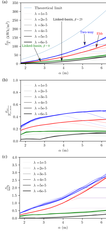
Figure 6: Sensitivity of tidal plant performance and configuration to amplitude ( \alpha ). (a) Spatially normalised annual energy \frac{E_{yr}}{A} , (b) generation efficiency relative to maximum potential energy \frac{E_{yr}}{E_{yr,max}} , (c) normalised turbine number per area for idealised ebb (—), two-way (—) single-basin and \beta = 0 (—), \beta = 25 (—) linked-basin configurations. The line width varies with the value of \lambda that is applied to constrain the introduction of hydraulic structures to a finite length of the impoundment.
