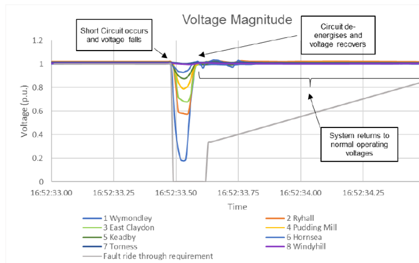
Figure 4 – Single-phase voltage profiles at various locations following the lightning strike (ESO, 2019).
