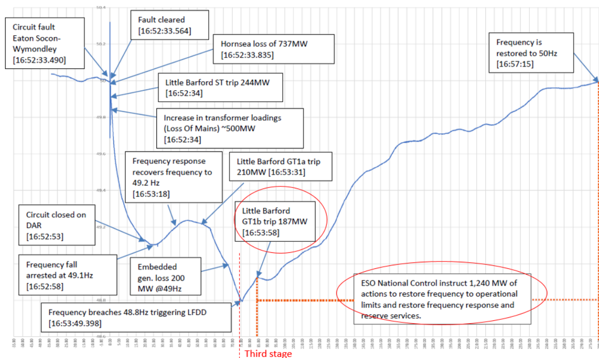
Figure 7 – Frequency trace: third stage - load shedding and restoration of 50 Hz (ESO, 2019)
