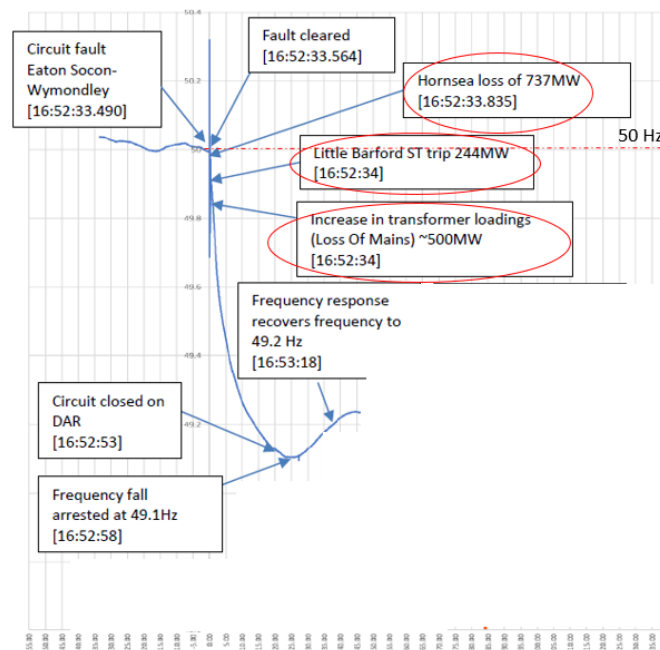
Figure 5 – Frequency trace at the first 45 seconds after the lightning strike (ESO, 2019).
