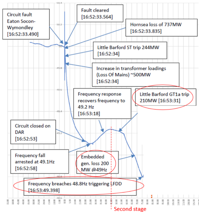
Figure 6 – Frequency trace: the second stage - next 11 seconds (ESO, 2019).
