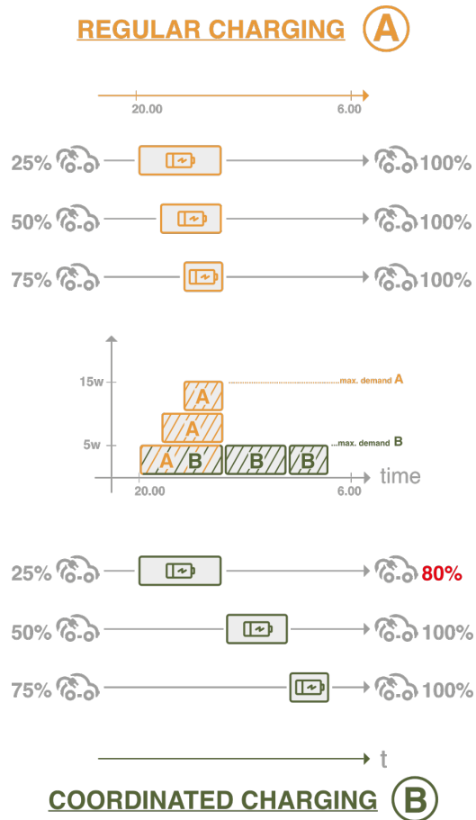
Fig. 11 Impact of regular and smart charging strategies on the peak power demand. Shown in the figure is the comparison between regular and smart charging resulted EV charging demand: peak power demand can be reduced significantly by combining mobility data and distributed control method.
