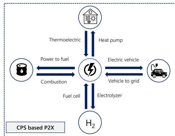
Fig. 4 Schematic of various Power-to-X (P2X) technologies applied in energy system. Shown in the figure are different technologies that could convert electricity into other energy end-users ( e.g. heat, gas, fuel and mobility) and vice versa.
