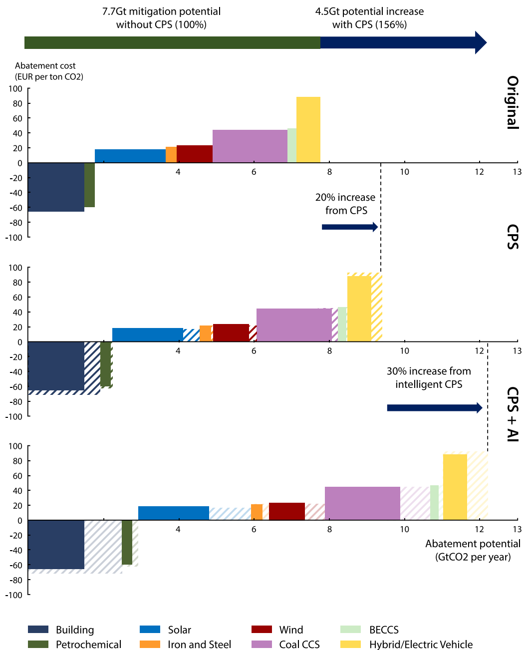
Fig. 17 Impact of CPS technologies on the marginal abatement cost of selected decarbonization technologies in energy transition. Shown in the figure is the marginal abatement cost of selected decarbonization technologies (represented by different colors) without CPS technologies (top 177 ), with CPS technologies (middle 34,119,180 ), and with intelligent CPS technologies (below 176,178,179 ).
