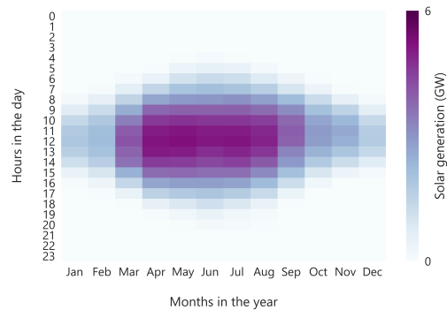
Fig. 7 Heat map of solar energy generation in the UK power system in 2017. Shown here is the UK power system average hourly solar power generation over 2017. Darker colors on the heat map represent higher values. Data shown in the figure is available from 116 .
