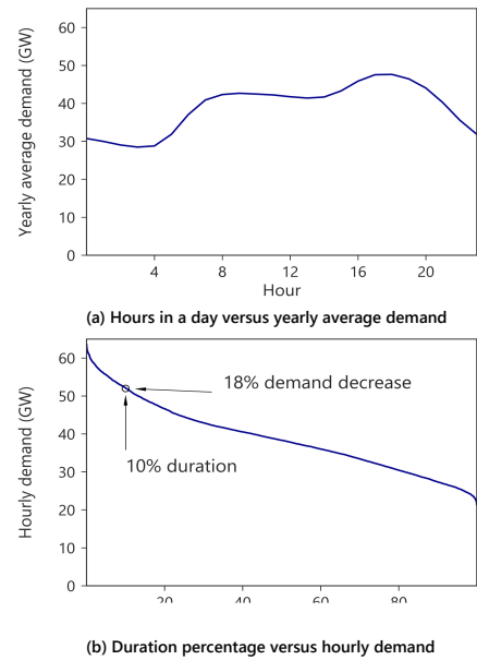
Fig. 8 UK power system demand profile in 2017. Shown here is the yearly average power system demand for different hours in the day (left); on the right is the percentage that various hourly demand accounts for. As can be seen, the top 18% demand only lasts for 10% during the year 116 .
