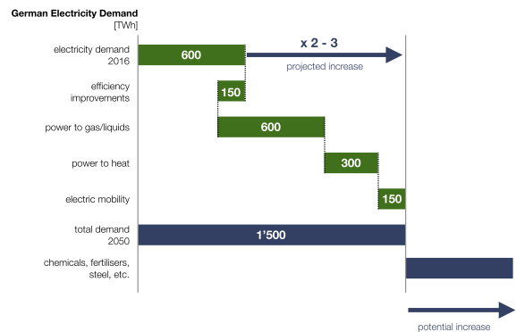
Fig. 10 Predicted electricity demand increase in Germany from 2016 to 2050 due to sector coupling between electricity sector and other end-users 57 .
