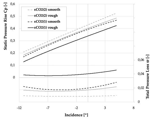
Fig. 8. Comparison between sCO_2(1) and sCO_2(2) cascades working with the same absolute roughness ( 5\mu m ).
