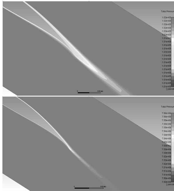
Fig. 17. Total pressure contours in partly similar NACA 65 compressor blade cascades operating on air (top) and supercritical carbon dioxide s\text{CO}_2(2) (bottom). Operating conditions reported in Table 3, with incidence i = -2.5^\circ .
