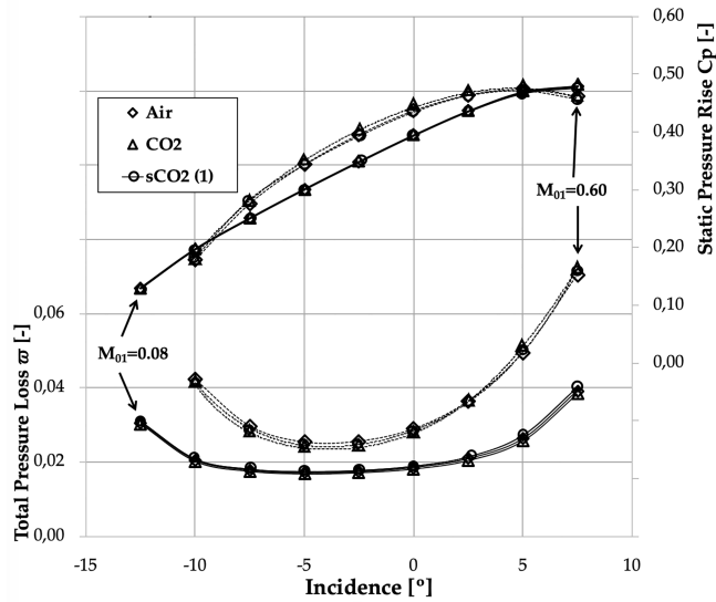
Fig. 12. Static pressure rise and total pressure loss for atmospheric air and atmospheric/supercritical CO 2 cascades. Dashed and solid lines correspond to M_{01}=0.6 and M_{01}=0.08 respectively.
