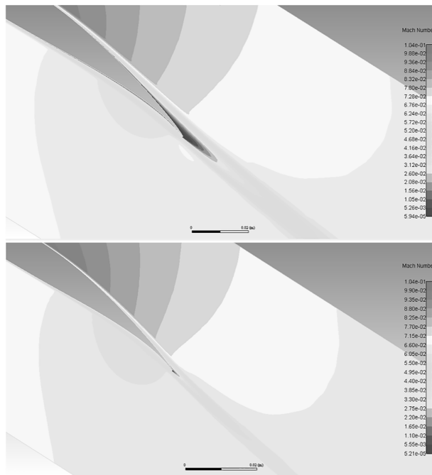
Fig. 18. Contours of Mach number in partly similar NACA 65 compressor blade cascades operating on air (top) and supercritical carbon dioxide s\text{CO}_2(2) (bottom). Operating conditions reported in Table 3, with incidence i = -2.5^\circ .
