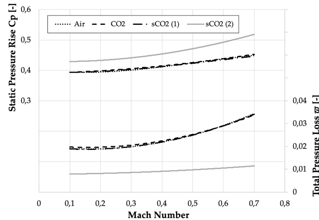
Fig. 13. Static pressure rise and total pressure loss for atmospheric air and atmospheric/supercritical CO 2 cascades.
