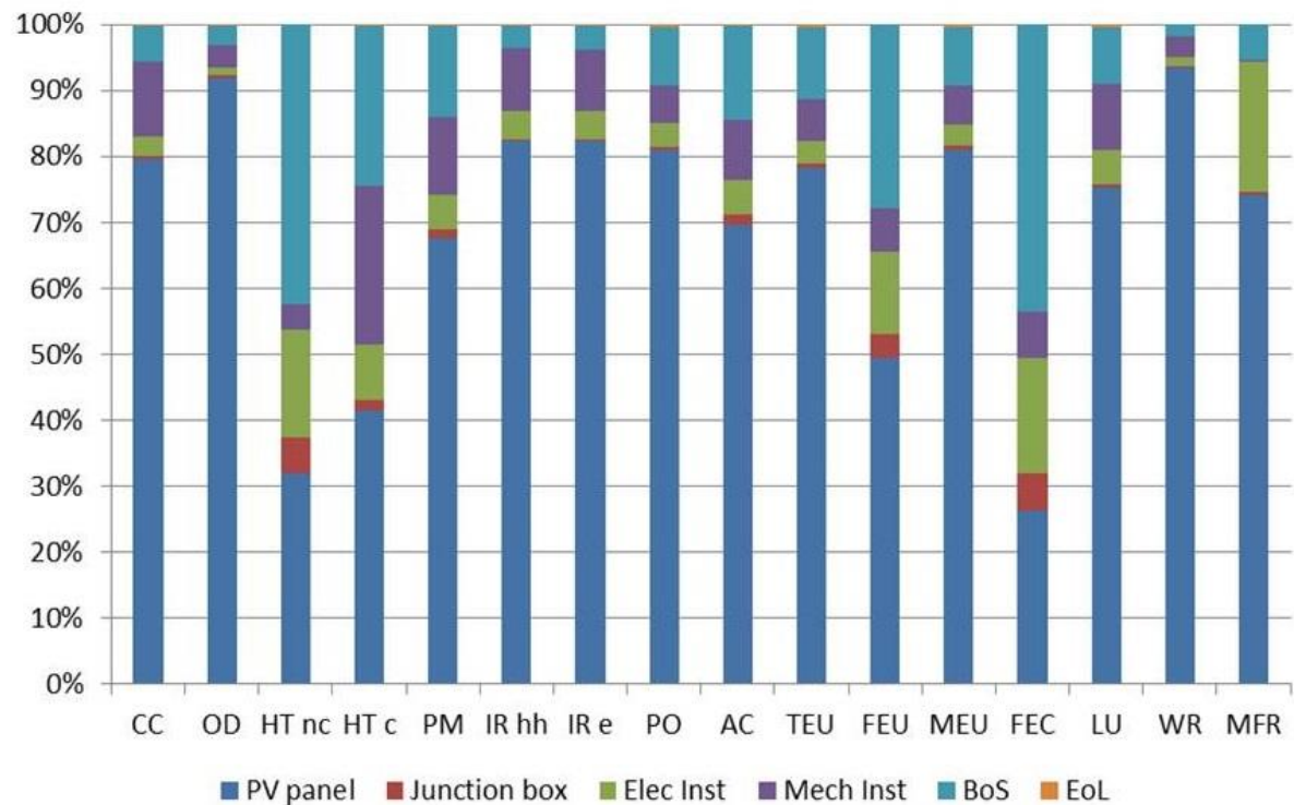
Figure 8. Contribution of each part in the EF of the BIPV.
