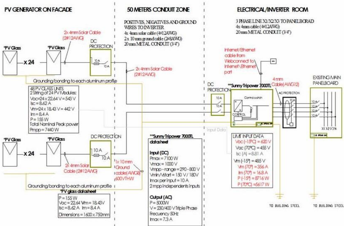
Figure 4. Single line diagram of the system.
