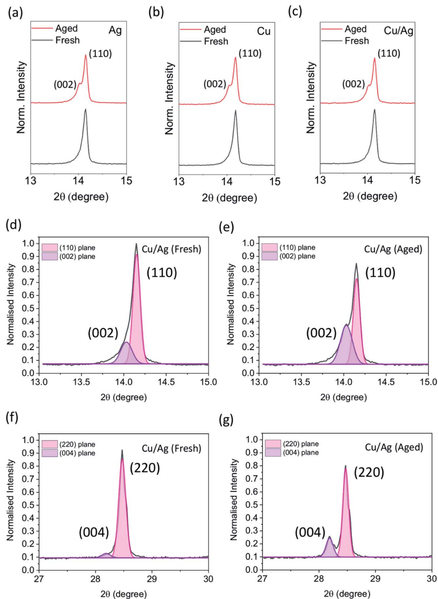
Fig. 5 XRD patterns of \text{MAPbI}_3 of devices with (a) Ag (b) Cu (c) Cu–Ag counter electrode before and after ageing under same condition in Fig. 1d. (d–g) The fitting plots of XRD data of \text{MAPbI}_3 before and after ageing.
