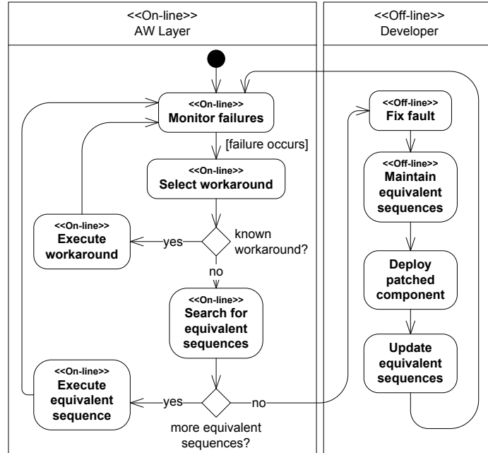
Fig. 8. Workflow of Activities in the Automatic Workarounds approach
