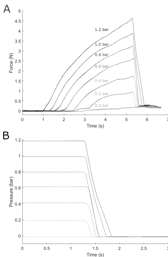
Fig. 5. The A) Force and B) Pressure responses for a PRR unit with an 11 mm aperture valve and internal pressure increasing from 0 bar to 1.2 bar by 0.2 bar.
