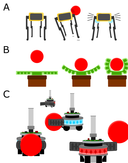
Fig. 9. Demonstrations of how to utilise the PRR units in existing robotic systems. A) PRR units act to stabilise a walking robot after it experiences lateral displacement due to impact. B) A biologically inspired, passive gripper that is able to capture objects it contacts. C) Swarm robots passively collecting items in an arena.
