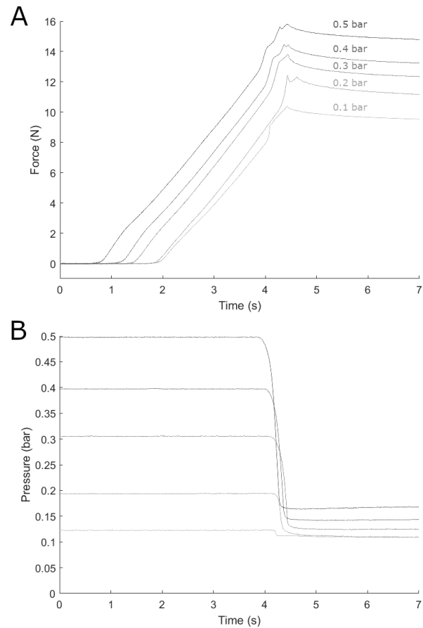
Fig. 7. The A) force and B) pressure responses for the coupled system, with 11 mm aperture PRR unit. Internal pressure increases from 0.1 to 0.5 bar in steps of 0.1 bar.
