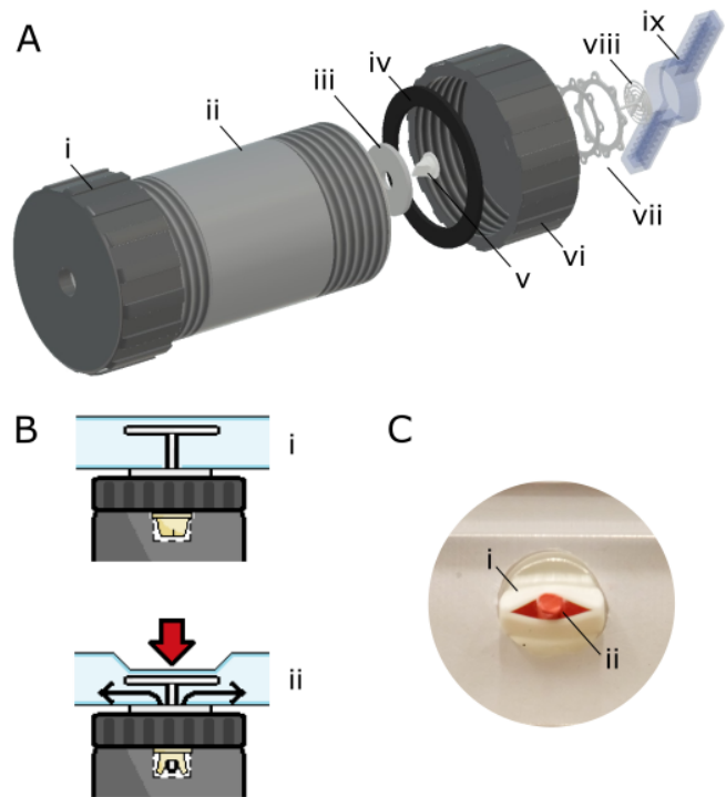
Fig. 2. Schematic of the PRR unit design. A) Exploded view diagram of the PRR unit. i) PVC threaded cap with hole for inlet. ii) PVC threaded pipe. iii) Acrylic disk for mounting the valve. iv) Rubber gasket. v) Silicone duck billed valve. vi) PVC threaded cap with hole for pin entry. vii) Mounting rings for the soft robotic actuator: one silicone to bond to the robot, one acrylic to mount to the cap. viii) 3D printed pin with flanged base to bond to soft robotic system. ix) Soft robotic actuator, in this instance a pneu-net. B) Principle of operation of the PRR unit. i) The system is combined and sealed with screws and silicone adhesive (with cut away to view valve). ii) The system is stimulated by pushing the pin into the PRR unit and allowing air to flow into the pneumatic network within the robot (with cut away to view valve opening). C) Front view of the valve mounted in the acrylic disk, with example of the pin opening the valve aperture. i) Soft valve. ii) A pin protruding through the valve aperture. A red pin was selected for clarity.
