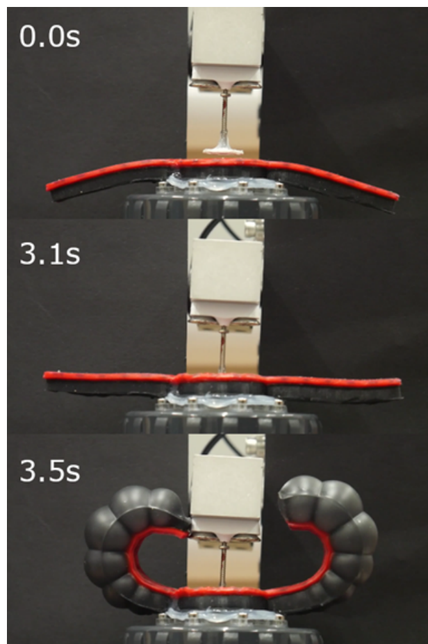
Fig. 1. Activation of a PRR unit. After 3.1s the force of the linear actuator is sufficient to trigger the PRR which then fully inflates the coupled pneu-net in under 0.5s.
