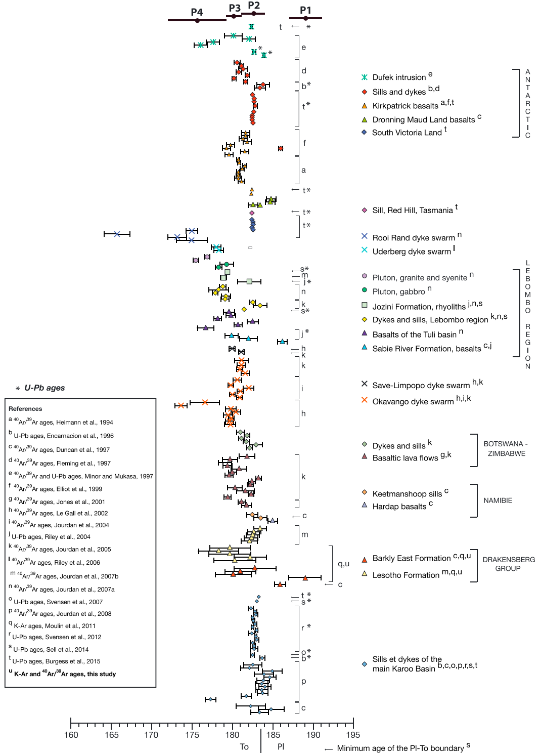
Figure 13. Compilation of 178 mineral separate 40 Ar/ 39 Ar (125), U/Pb (48), and K-Ar (5) ages (at the 1σ level) obtained for the Karoo-Ferrar magmatic province. All 40 Ar/ 39 Ar are intercalibrated using the new recommended age of 28.201 Ma [Kuiper et al., 2008] for the FCTs standard. We define four eruptive phases (P1 to P4; see text). Phase P1 is of minor importance and possibly of short duration; Phase 2 coincides with the major environmental and climatic perturbations, suggesting that it is related to the emplacement of the main part of the Karoo basalts and the release of large amounts of volcanic and thermogenic gases. Phase 2 may be divided into two subphases to fit the environmental events (see discussion). Phase 3 corresponds to moderate volcanic activity. Phase 4 represents the final period of volcanism, stretching from 179 to 175 Ma, mainly observed in Leleombo (South Africa) and Ferrar (Antarctica).
