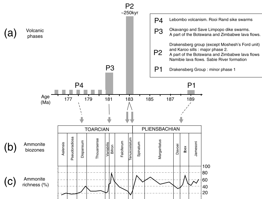
Figure 15. (a) The eruptive scenario proposed for the volcanic province (see text for more details). Possible correlations between crises and environmental perturbations linked to emplacement of the Karoo-Ferrar province near the Pliensbachian-Toarcian boundary. Height and width of rectangles represents roughly the importance and duration of the volcanic activity respectively. (b) Paleontological ammonite zones. (c) Variations in ammonite species richness.
