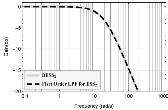
Figure 17. DGU 2 filter system response estimate.
