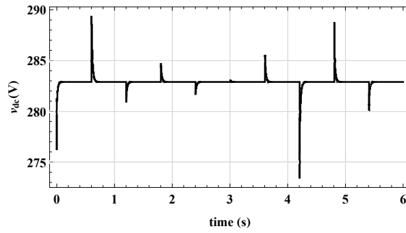
Figure 5. dc-link voltage for \omega_{cut-off} = 1000 \frac{\text{rad}}{\text{s}} .
