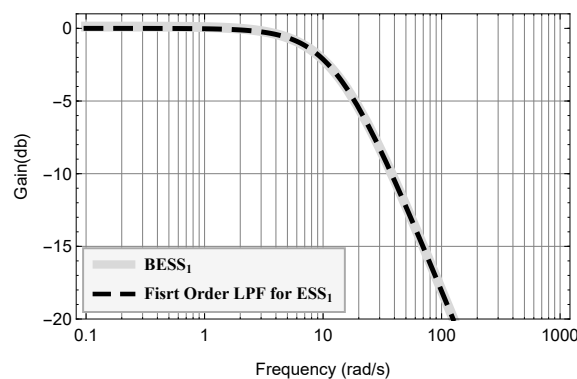
Figure 16. DGU_1 filter system response estimate.
