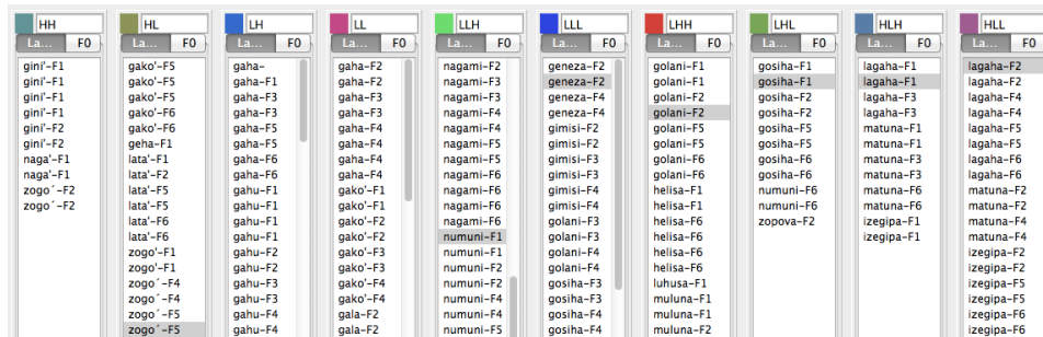
FIGURE 7: Classification of Alekano words from six sentence frames, controlling for the tone on preceding and following syllables, with frame identifiers displayed
