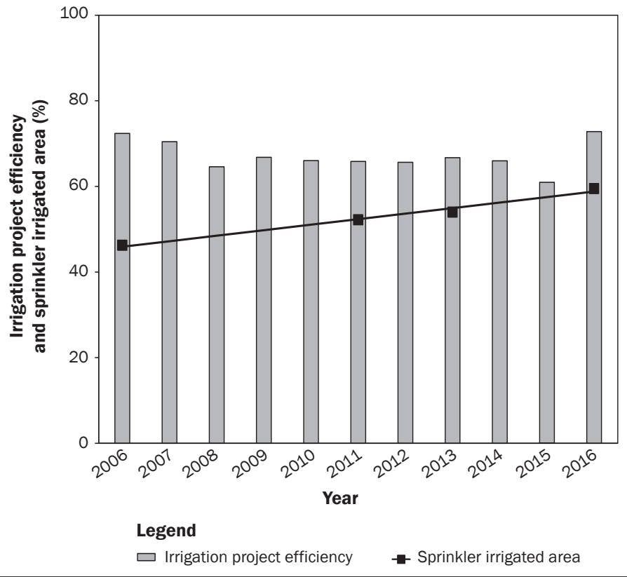
Figure 2 Irrigation project efficiency based on ETIdaho and relative amount of sprinkler irrigated cropland for the Twin Falls Canal Company irrigation project.
