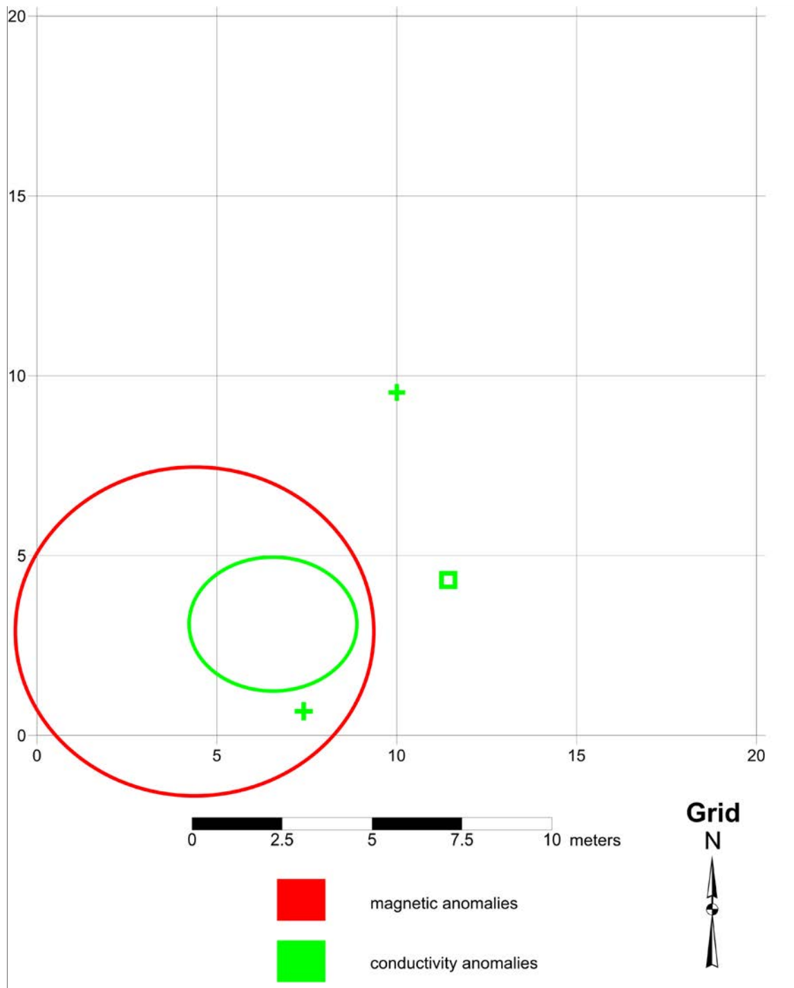
Figure 30. Combined geophysical survey data from Area C.
