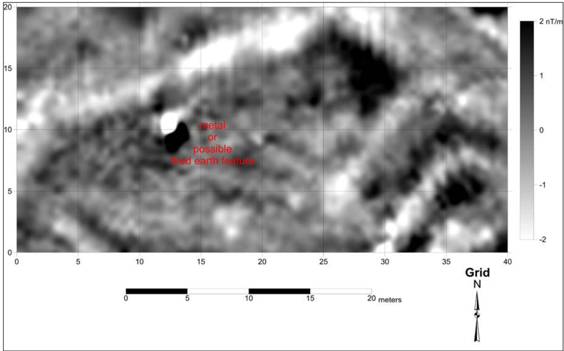
Figure 23. Interpretation of the magnetic data from Area B.
