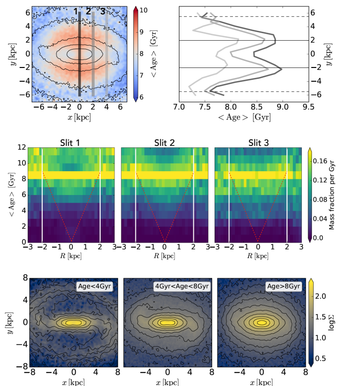
Fig. 14. Results from Auriga simulations. The top-left panel shows a face-on mass-weighted age map of halo 18 from the Auriga sample, over-plotted with three vertical lines that indicate the cuts to extract the data shown in the other panels. The bar major axis is horizontal. The top-right panel shows the mean stellar age profiles along the cuts. The middle row presents SFHs diagrams for each of the cuts (the left panel corresponds to the dark slit and the rightmost panel corresponds to the light grey slit). The axis and the colour-coding are the same as in our observations shown in Fig. 13. The white solid lines mark the edges of the bar and the red dashed line indicate the V-shape that we discuss in the main text. The bottom row shows face-on surface density projections of stars in the bar in three different age bins as indicated in the top right corner of each panel. We see that younger ages cluster along the bar major axis compared to older ages which have a rounder shape.
