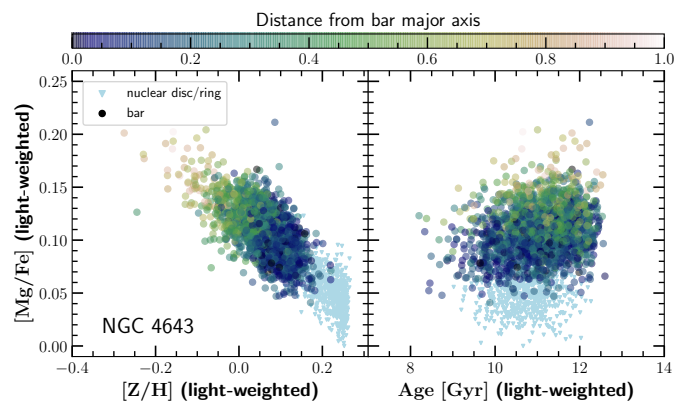
Fig. 12. Comparison between light-weighted [\text{Mg}/\text{Fe}] , metallicity and age of the stellar populations in the bar of NGC 4643. Each point corresponds to one Voronoi bin as shown in Fig. 5. Bins are coloured by their distance to the bar major axis and only bins within the bar are shown. Bins within the nuclear structure are marked with different symbols and in light blue. These plots are shown for all galaxies in Figs. A.1 and A.2.
