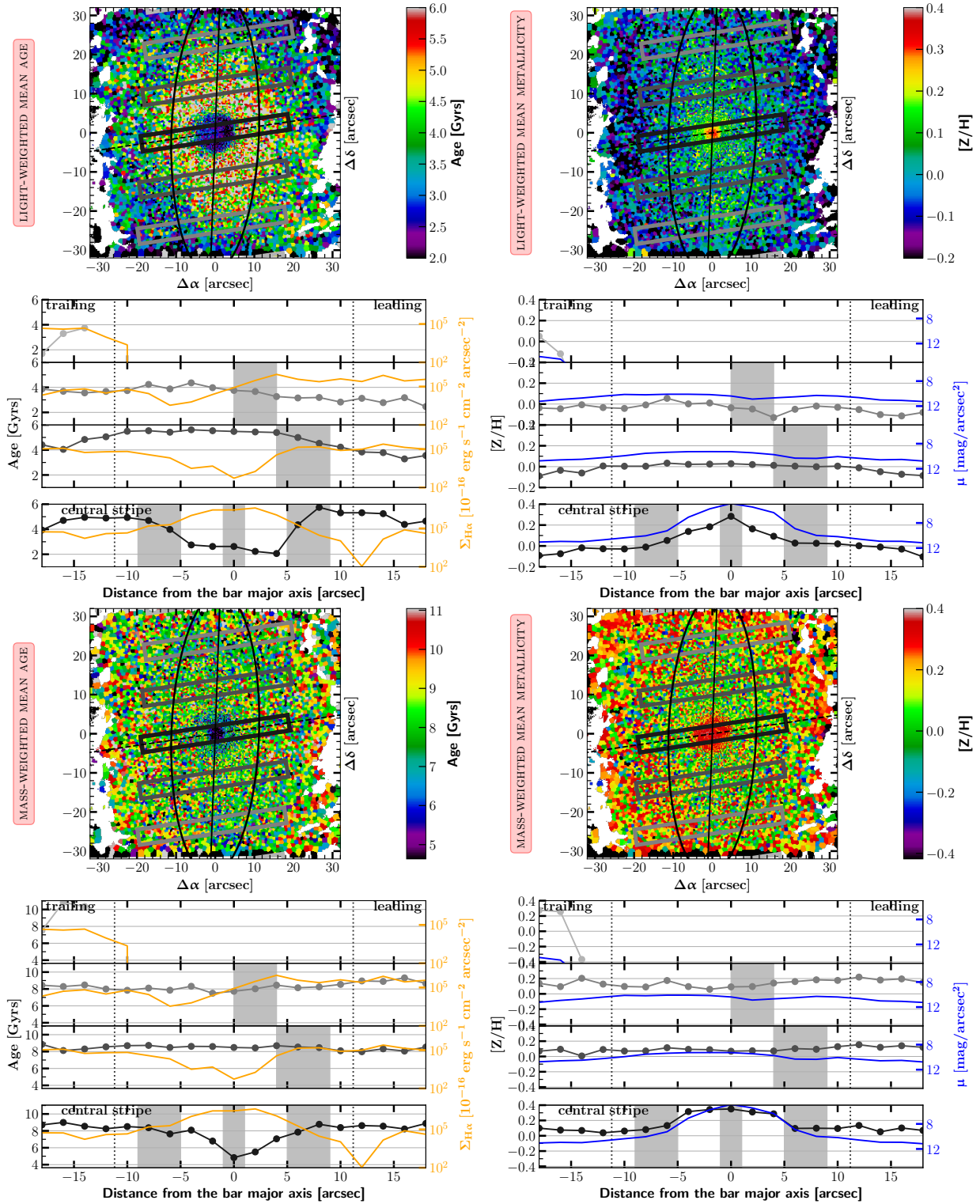
Fig. C.2. Same as C.1.
