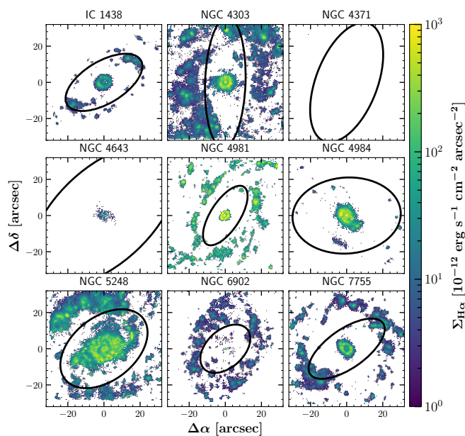
Fig. 2. Dust-corrected H\alpha maps for the complete sample. Only fluxes with S/N_{H\alpha} > 5 and S/N_{H\beta} > 5 are shown. Black ellipses outline the approximate extent of the galaxy bar. NGC 4371 does not have any H\alpha above the S/N cut.
