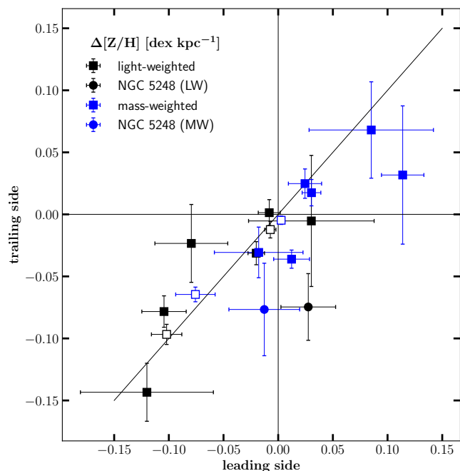
Fig. 11. Same as Fig. 10 but for gradients of mean stellar metallicities.
