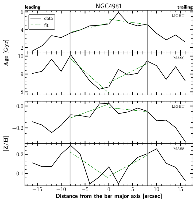
Fig. 9. Very simplified and shortened version of Figs. C.1-C.9 as an example for NGC 4981. Shown are light- and mass-weighted age and metallicity profiles along cut #2 (see Fig. 8) perpendicular to the bar major axis. The width of the cuts is 4'' and bins are equally spaced every 2'' along the cuts. The two cuts #2 are averaged in anti-parallel direction as shown in Fig. 8. Vertical lines mark the edges of the bar. Linear regression fits from the major axis to the edges of the bar are shown in green. The slopes of these fits are tabulated in Table 3 and plotted in Figs. 10 and 11.
