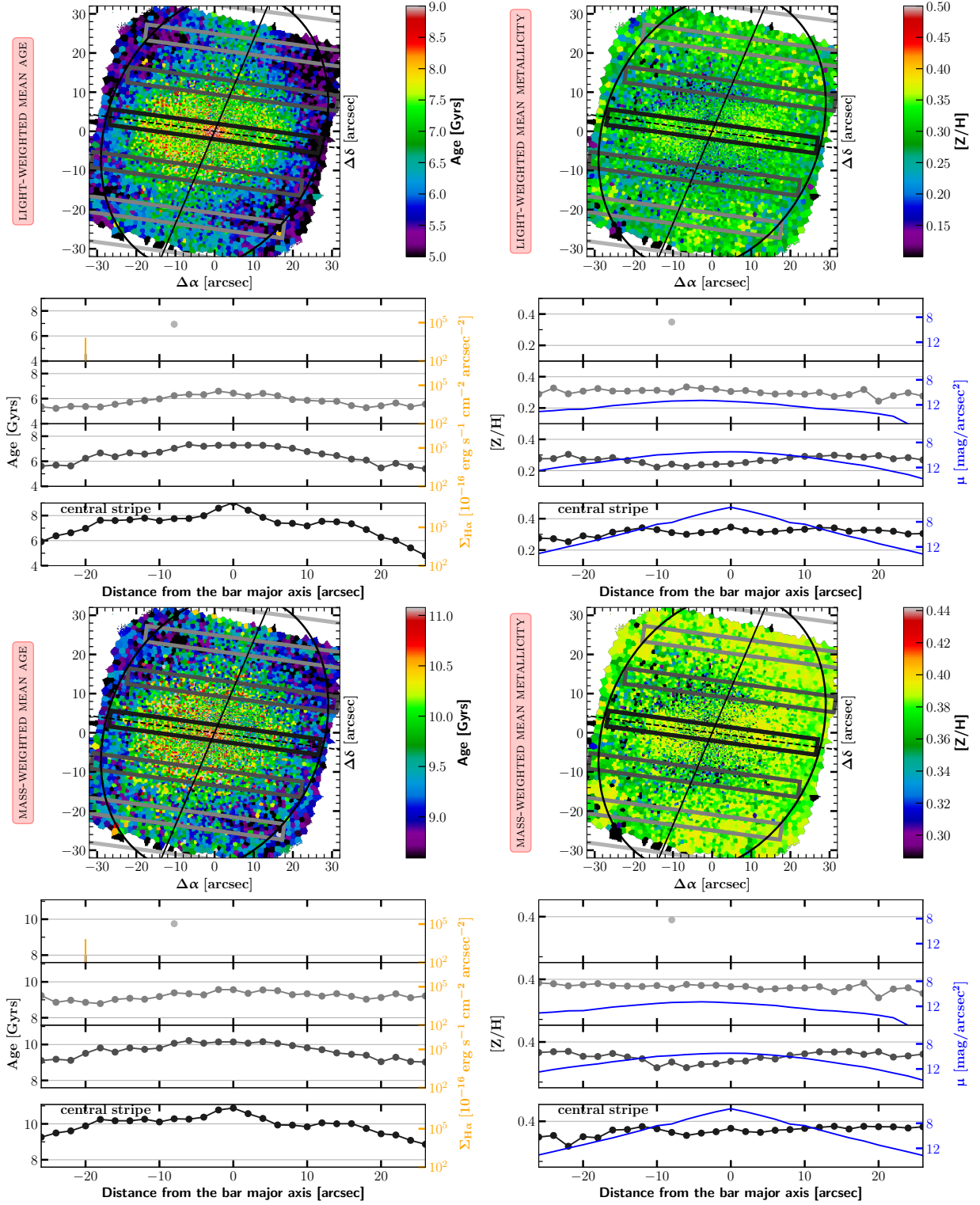
Fig. C.3. Same as C.1.
