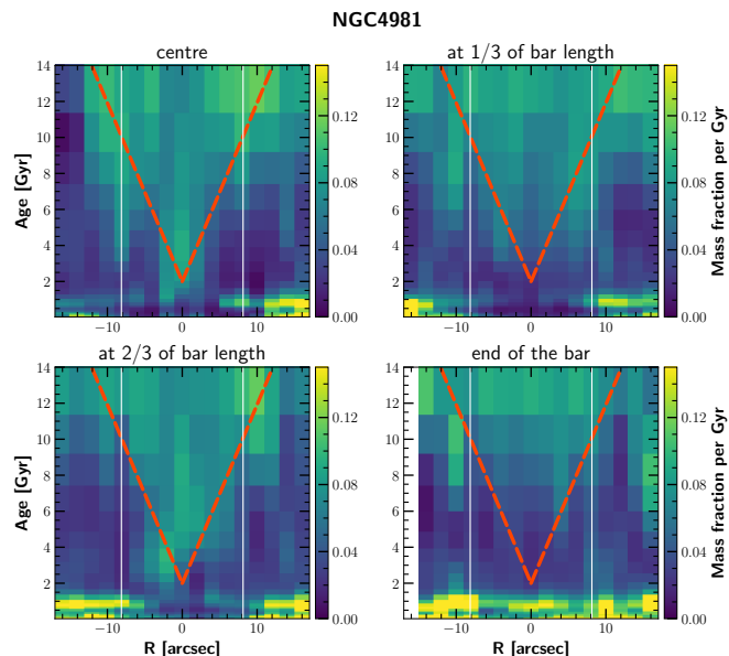
Fig. 13. SFHs of NGC 4981 along the cuts illustrated in the sketch in Fig. 8. and in the Figs. C.1-C.9. Each panel shows one of the four cuts. The x-axis shows the distance to the bar major axis along the cut and the y-axis the age of the population. Colour-coded is the fraction of stellar mass that is at a certain position and was formed at a certain time. The mass is normalised within each spatial bin (vertically in this diagram). The mass fractions are further divided by the size of the bin on the y-axis to correct for non-equally spaced bins on the linear age axis. White vertical lines mark the edges of the bar. Red lines are plotted on top to indicate the ‘V-shape’ discussed in the text.
