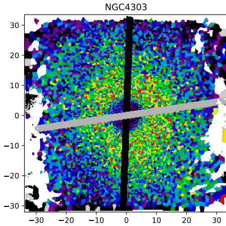
Fig. B.1. Sketch to visualise the procedure of extracting age and metallicity profiles along the deprojected bar major and minor axis. Shown is here a map of light-weighted Voronoi-binned mean ages from NGC 4303. Overplotted are pseudo-slits that were used to extract the profile of the major axis (black stripe) and minor axis (grey stripe).
