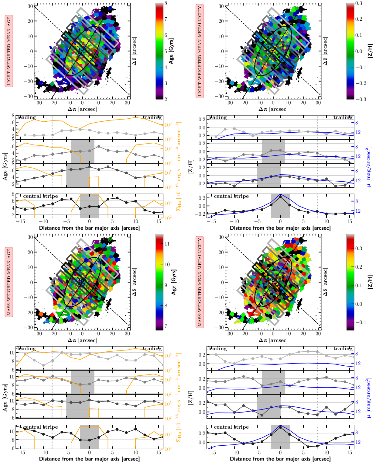
Fig. C.5. Same as C.1.
