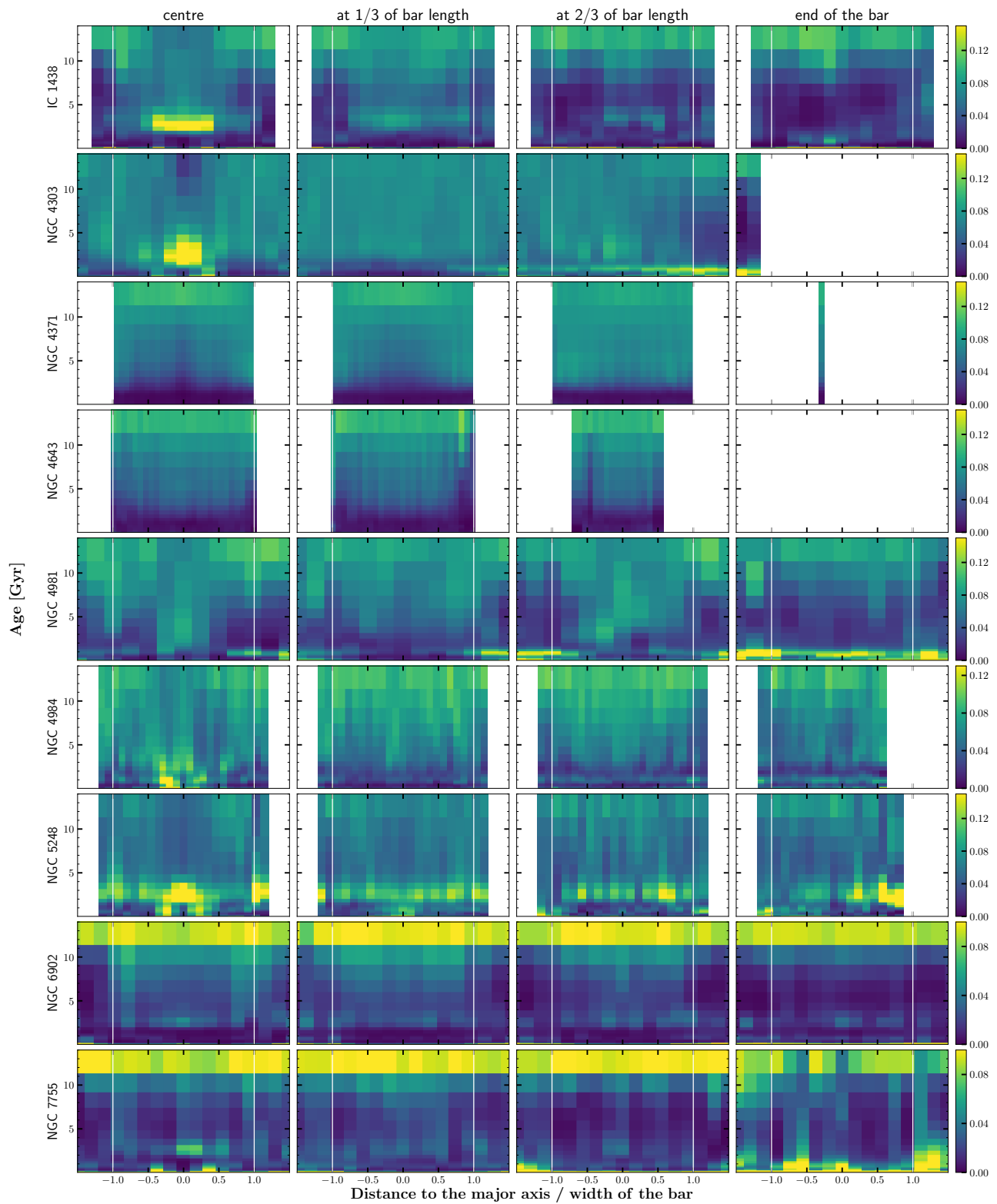
Fig. D.1. SFHs of the complete sample. Details of the figure are the same as in Fig. 13. The four panels are shown here from left to right in one row for each galaxy. In some cases the colour bar is stretched in order to show fainter details that allow to recognise the ‘V-shape’ discussed in the main text.
