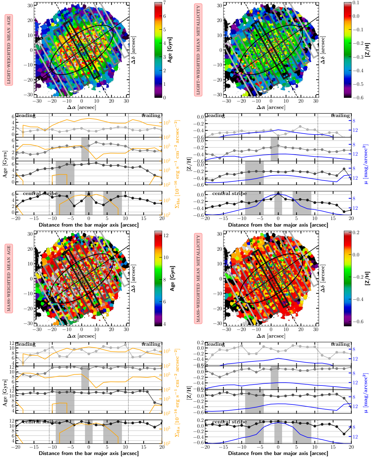
Fig. C.9. Same as C.1.
