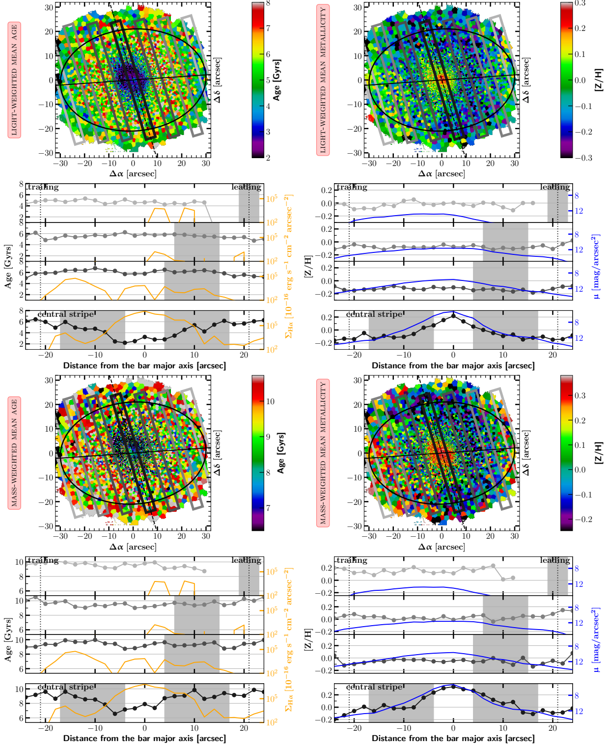
Fig. C.6. Same as C.1.
