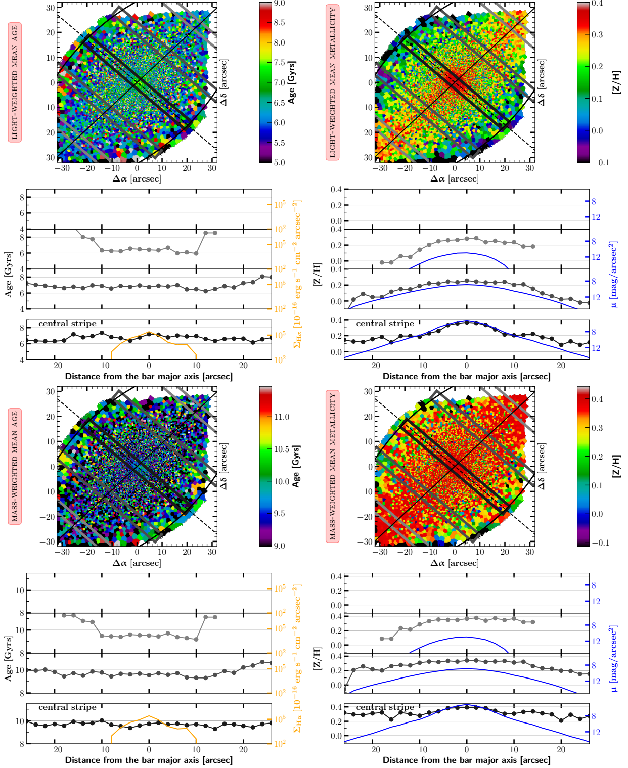
Fig. C.4. Same as C.1.
