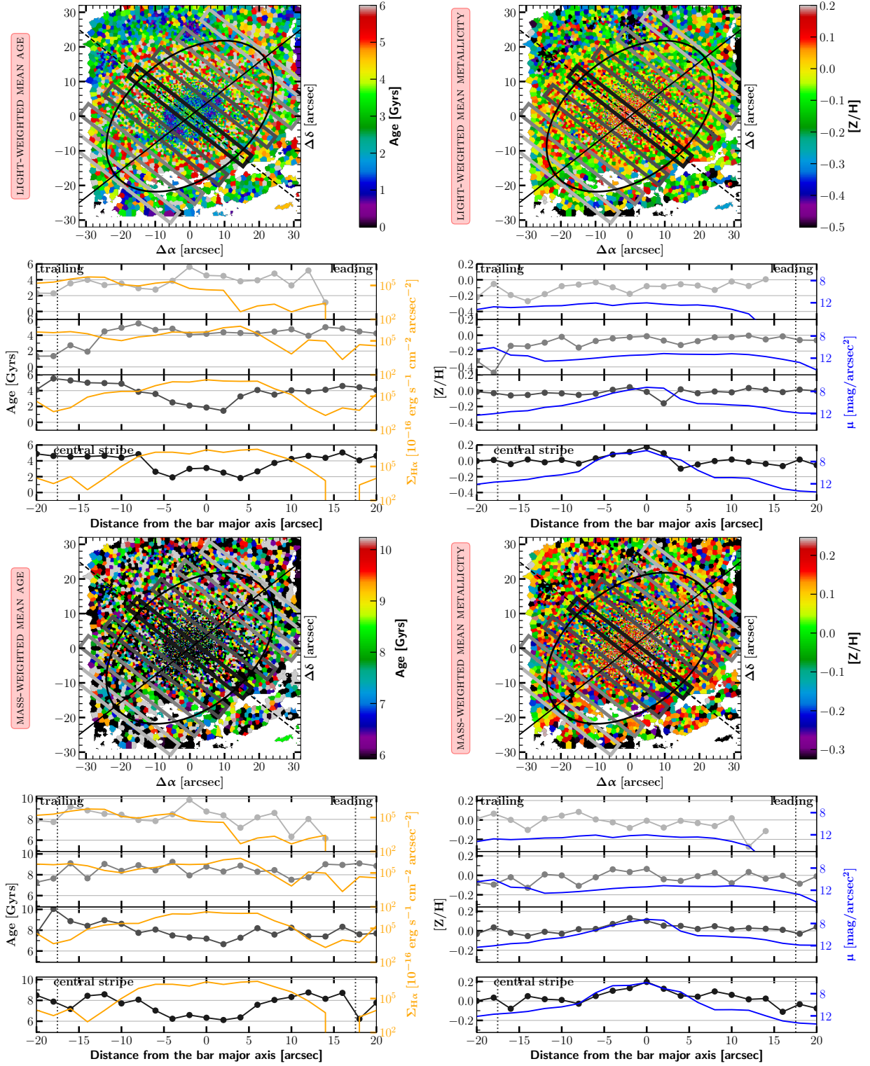
Fig. C.7. Same as C.1.
