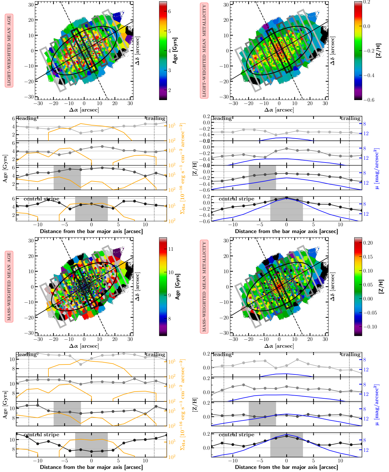
Fig. C.1. Light- and mass-weighted mean ages and metallicities. The figure splits into four quarters. On the left we show ages and on the right we show [Z/H] . The top shows light-weighted values, the bottom mass-weighted. In each quarter we show a 2D map of Voronoi-binned mean values overplotted with an outline of the bar (black ellipse), the bar major axis (solid line), the minor axis (dashed line) and outlines of the cuts from which we derive the profiles shown below (empty rectangles). Below each map, in four panels, we plot averaged profiles extracted from the corresponding cuts shown in the map. The shades of grey of the profiles correspond to the grey of the rectangles in the map. Also shown are H\alpha (orange line), total surface brightness (blue line) and the approximate position of dust lines (grey area). Vertical grey dotted lines mark the edge of the bar assuming for simplicity a rectangular shape. Further details can be found in the text.
