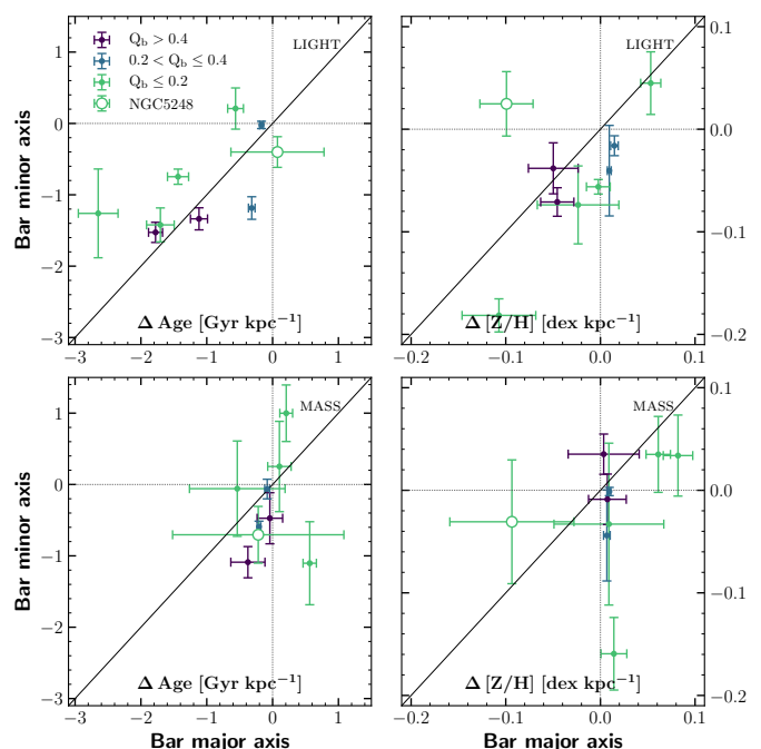
Fig. 7. Gradients of deprojected age and metallicity profiles for light- and mass-weighted mean values along the bar major and minor axes. An example of such profiles is shown in Fig. B.2. Gradients are measured between the second inner break and the bar length as seen in the aforementioned figure and discussed in the text. The minor axes are extended into the disc within the bar radius. Points are grouped into three bins of bar strength Q_b . NGC 5248 is an outlier and shown separately. Error bars show standard errors from the linear regressions to the profiles.
