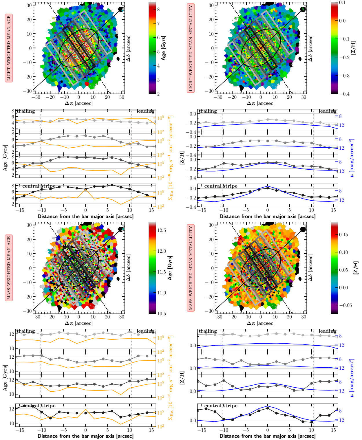
Fig. C.8. Same as C.1.
