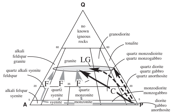
Figure 2. IUGS classification for quartz-bearing felsic rocks showing the differentiation paths followed by various granitic plutons—granitoids of Cordilleran batholiths; C—Caledonian batholiths; F—ferroan granites; LG—peraluminous leucogranites; Q—quartz; A—alkali feldspar; P—plagioclase. From Frost and Frost (2014).
