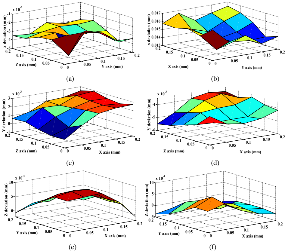
Fig. 9. Surface irregularity effect on a 200 \mu\text{m} 200 \mu\text{m} spatial grid. a) Negative X-probing, b) positive X-probing, c) positive Y-probing, d) negative Y-probing, e) negative Z-probing in X+ region and f) negative Z-probing in X- region of the artefact
