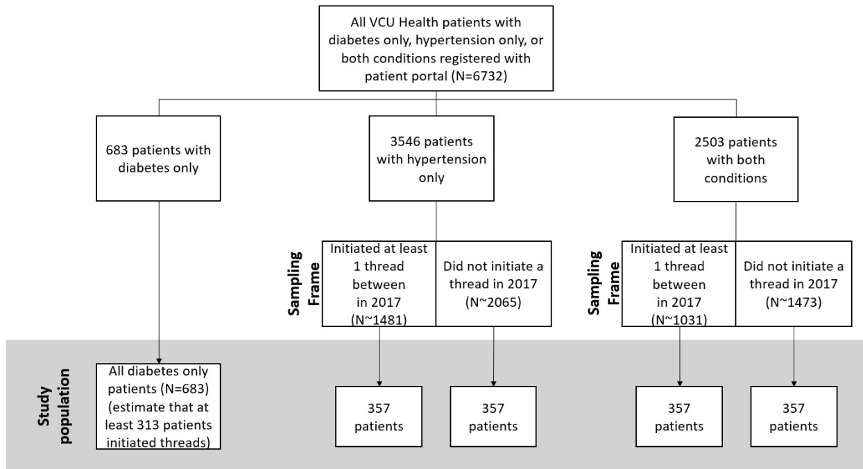
Figure 2-4. Sampling Strategy
